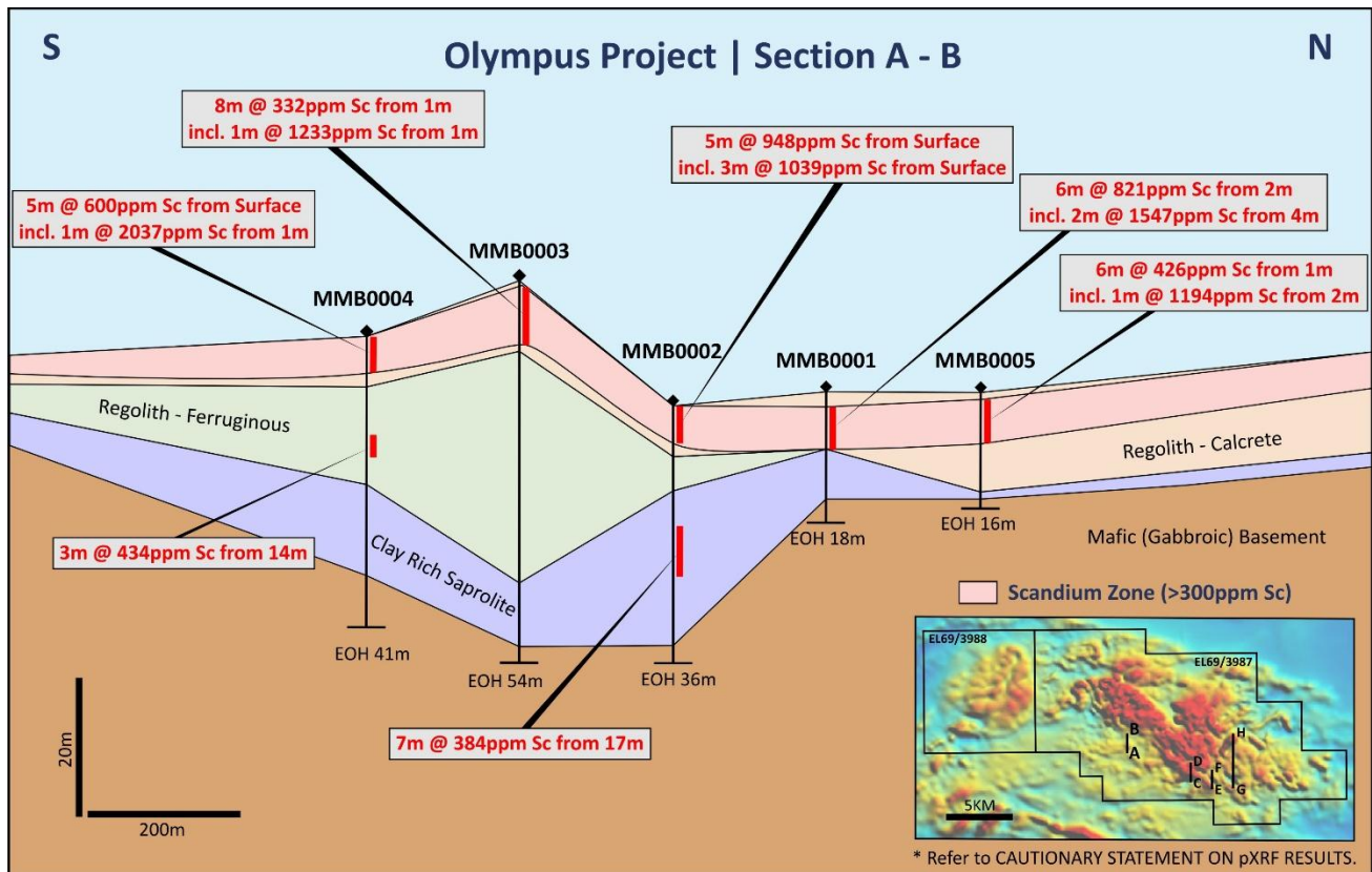
Figure 5: Olympus RAB Line A-B highlighting scandium intersections
