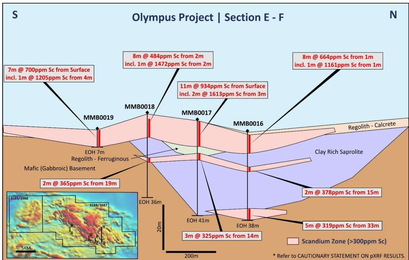
Figure 6: Olympus RAB Line E-F highlighting scandium intersections.
