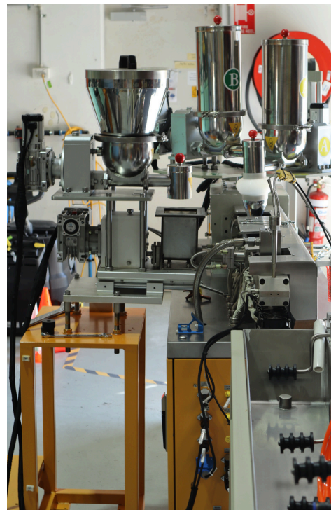
Figure 2: Twin-screw extruder used for graphene-polymer compounding
