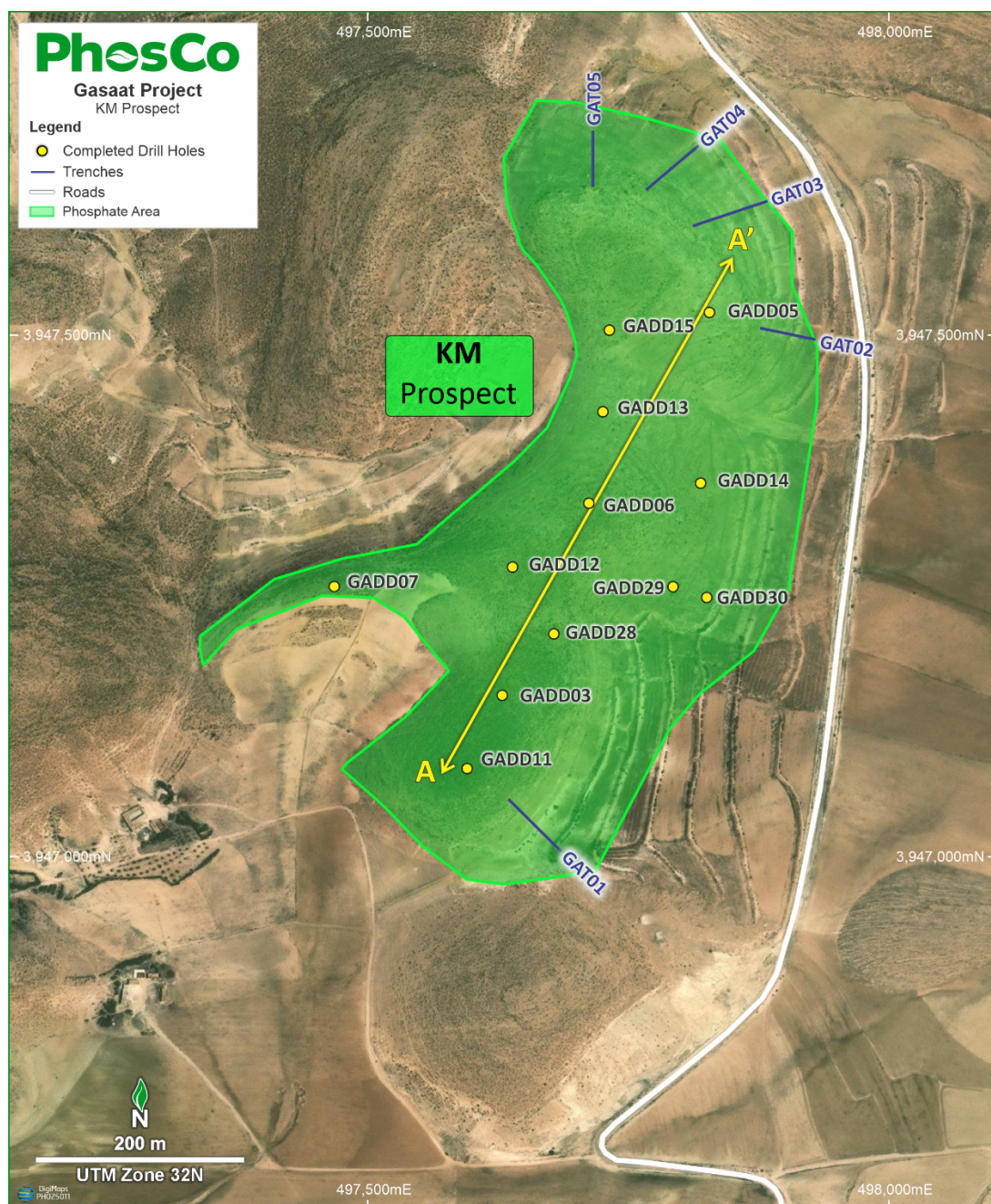
Figure 4. KM prospect showing location of drill holes and trenches
