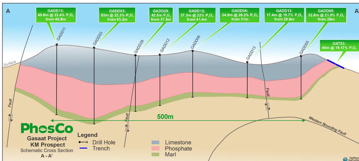
Figure 5. KM section A-A' showing generalised geology as determined by drilling, trenching and outcrop mapping, with drill holes projected onto section
