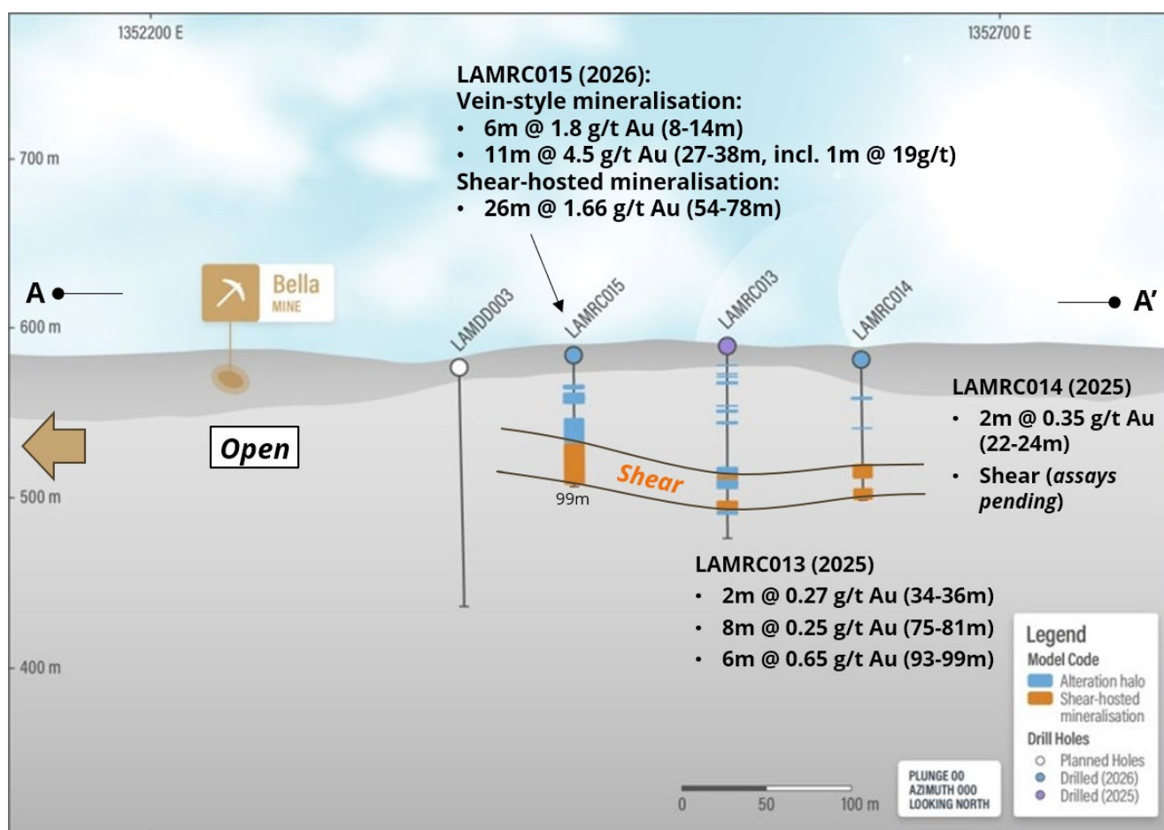
Figure 1 - Bella Prospect, cross section – including LAMRC015 and planned drillholes LAMDD003 and LAMDD004.
