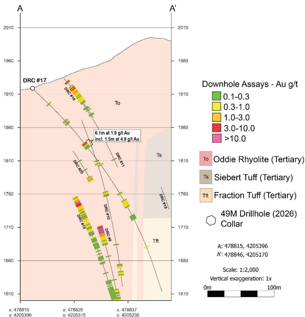
Figure 4: Cross-Section Showing Hole DRC#17
