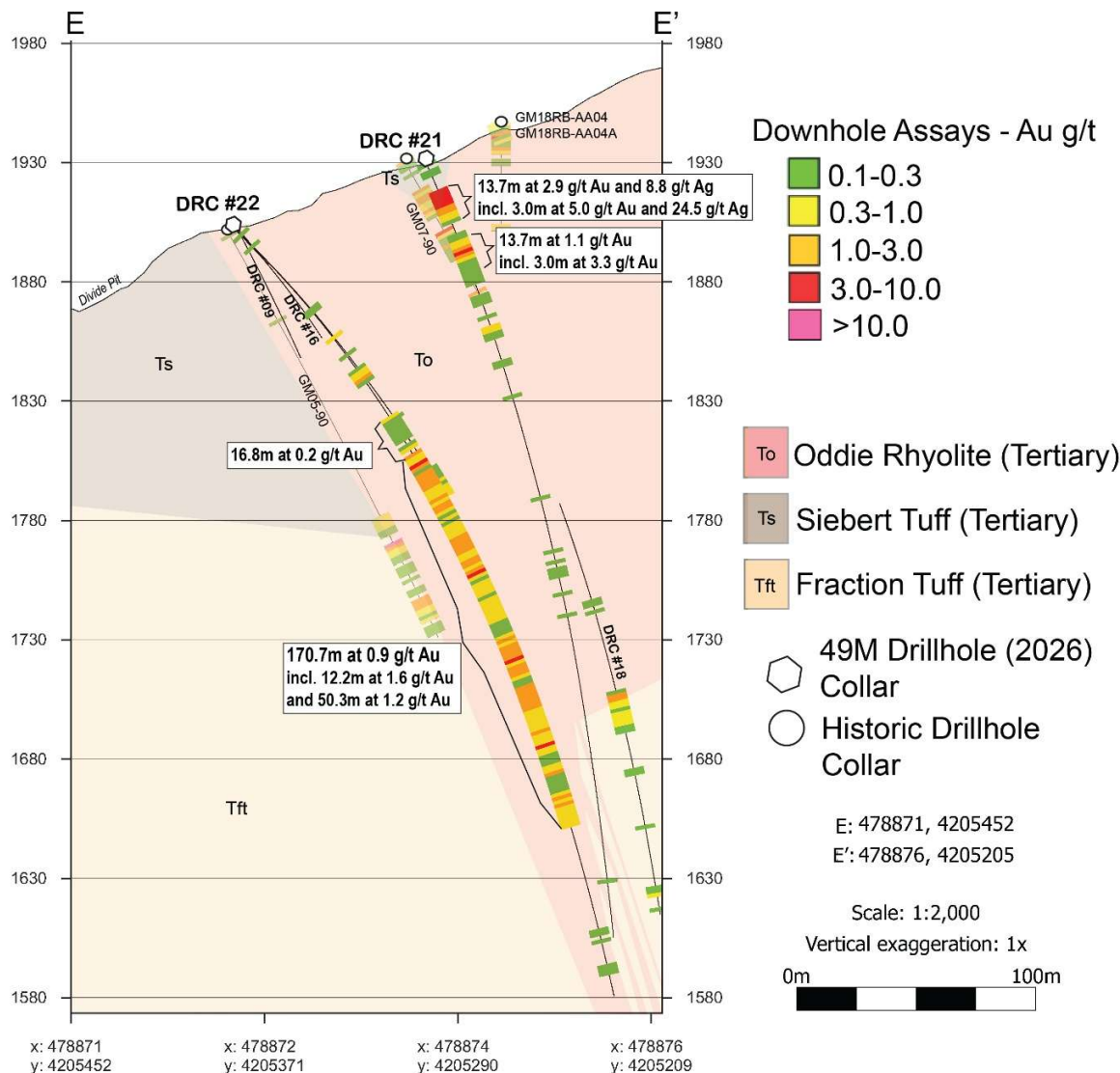
Figure 3: Cross-Section Showing Hole DRC#21 & DRC#22
