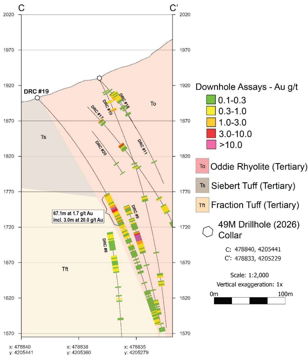
Figure 2: Cross-Section Showing Hole DRC#19
