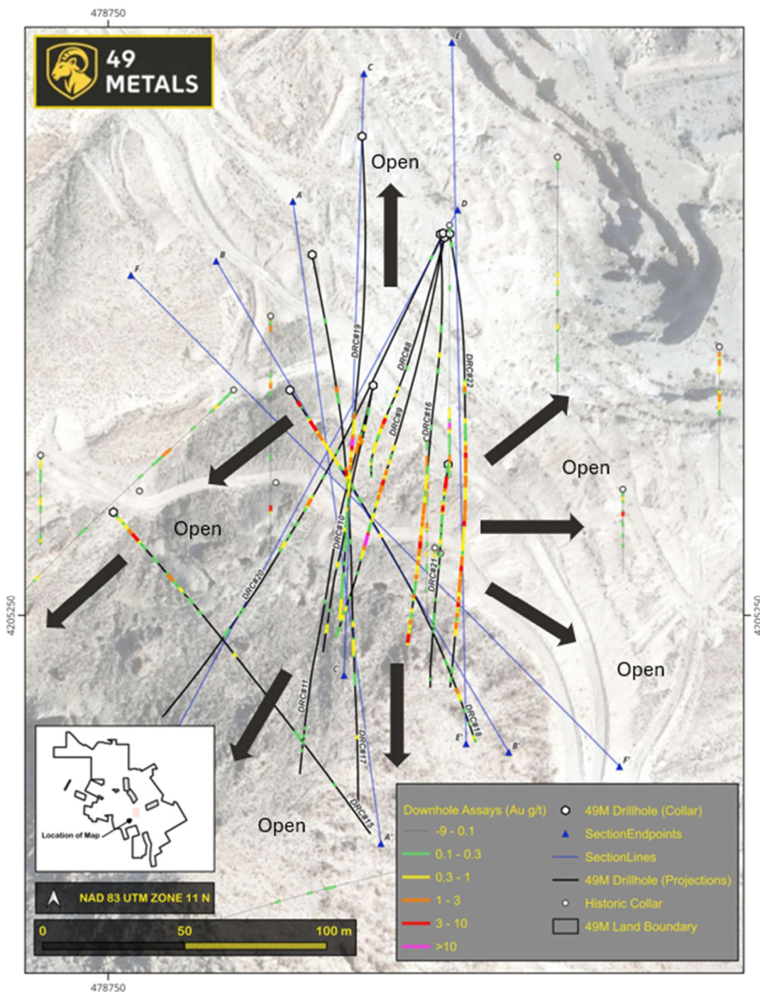
Figure 1: Collar Locations, Adit Zone Discovery Area
