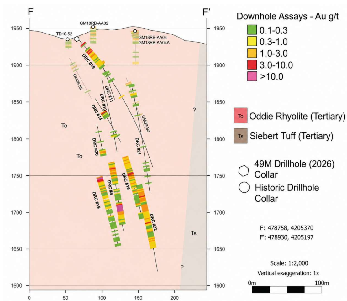
Figure 6: Long Section of the Adit Zone Discovery Area
