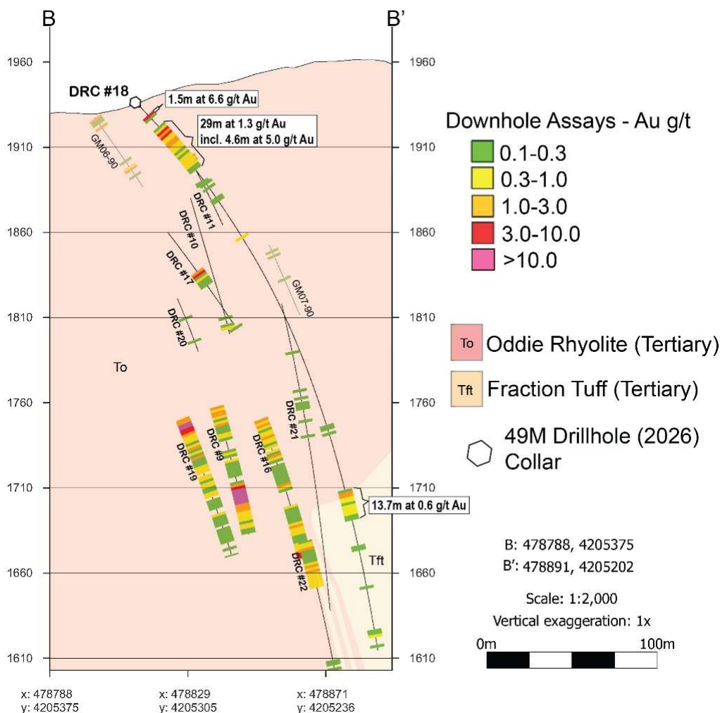
Figure 5: Cross-Section Showing Hole DRC#18
