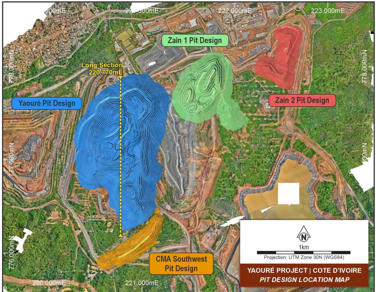
Figure 3: Yaouré Gold Mine Project Areas
