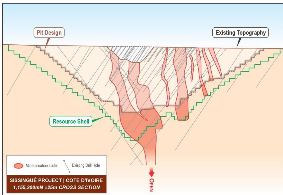
Figure 6: Cross section of Bagoé Ore Reserve pit design with Mineral Resource shell
