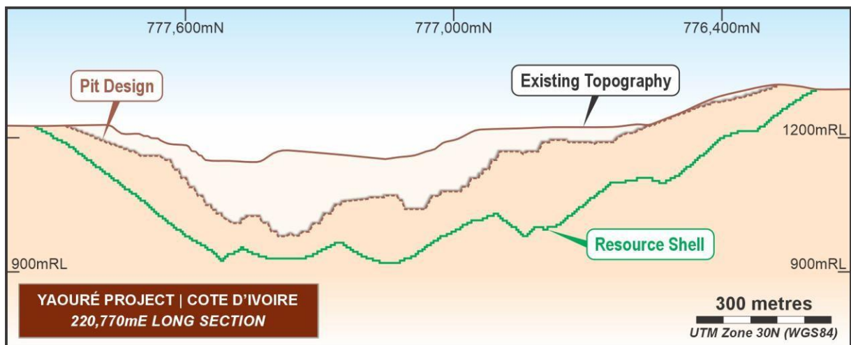
Figure 4: Yaouré Open Pit long section showing Ore Reserve design and Mineral Resource shell
