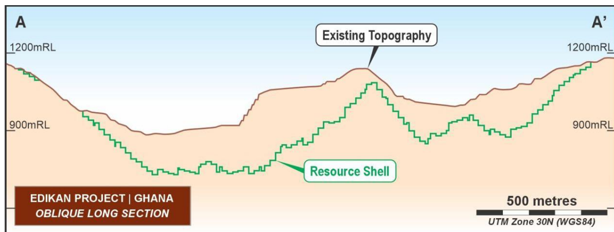
Figure 8: Oblique long-section showing AG-Fobinso (AGF) pit void and Mineral Resource shell
