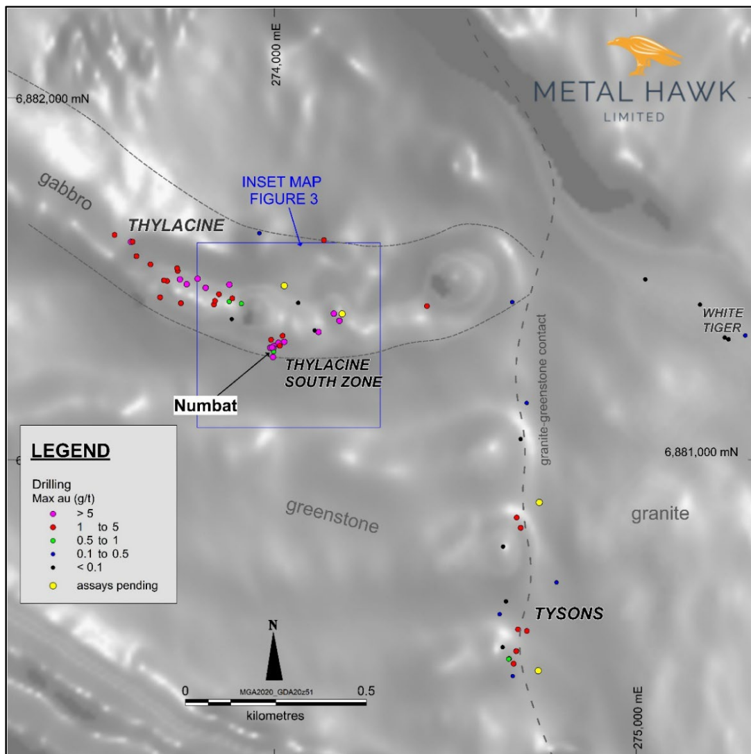
Figure 5. Leinster South drilling July 2026 (max Au g/t)
