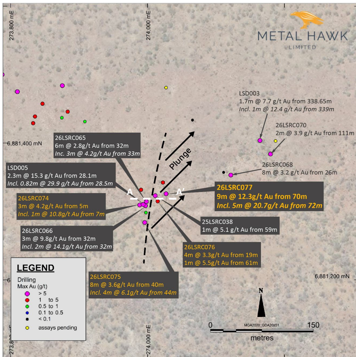
Figure 3. Thylacine south zone drilling (max Au g/t) - holes intersecting the Numbat lode labelled white (previous results) and orange (new results)
