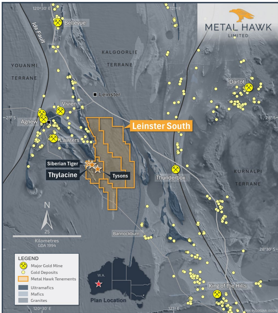
Figure 6. Leinster South Project
