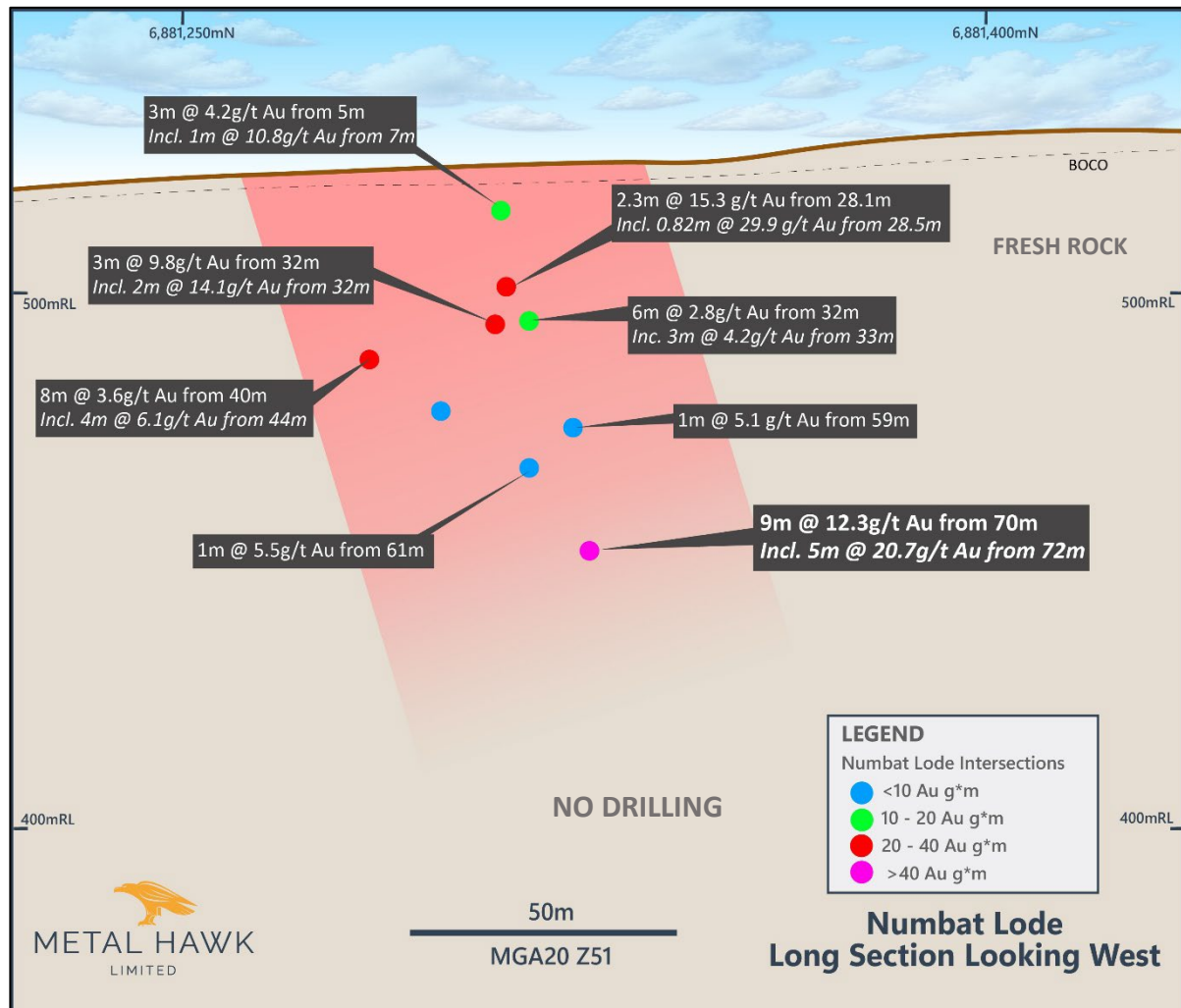
Figure 4. Long section looking west, showing Numbat lode drill intersections
