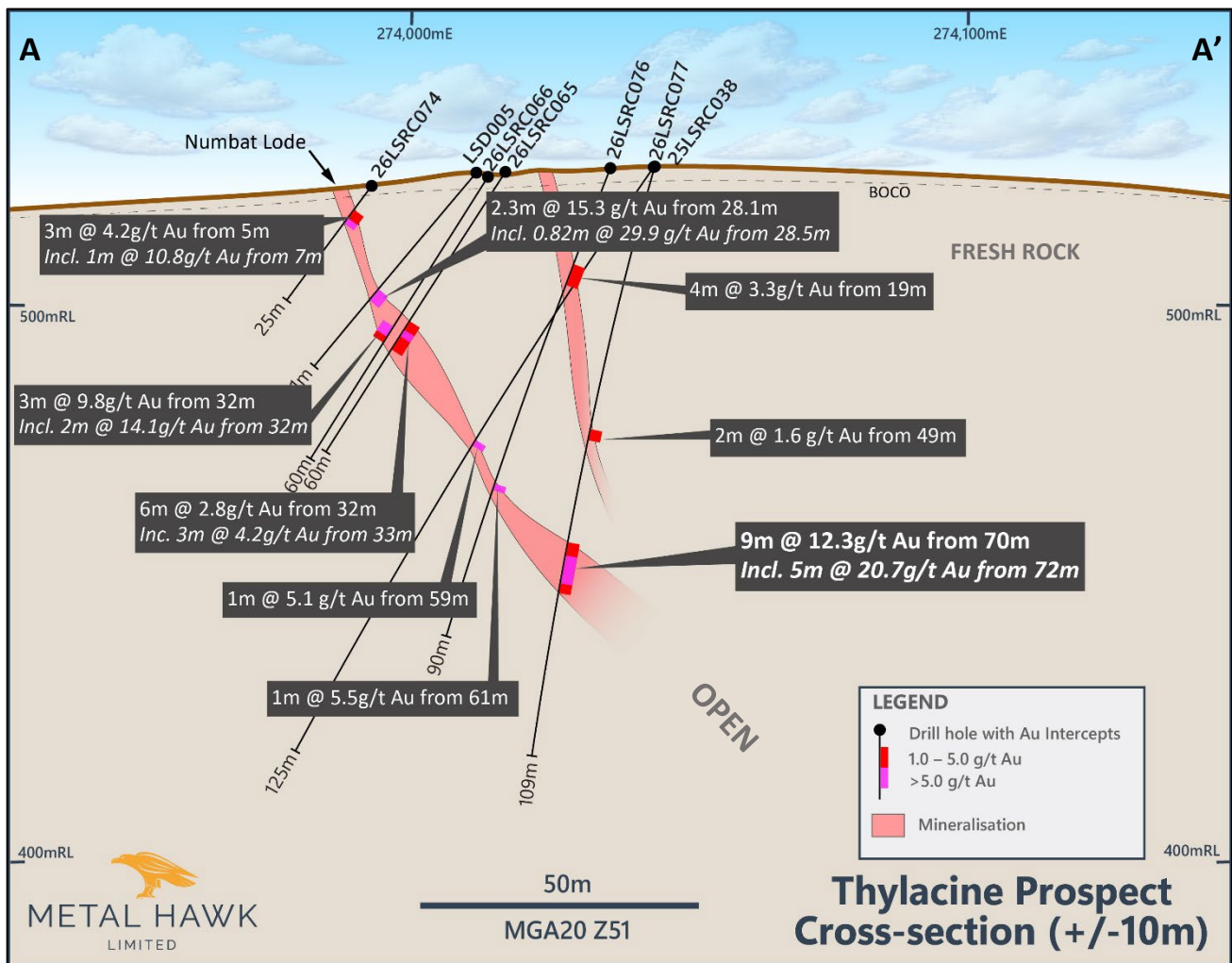
Figure 2. Cross-section of the Numbat lode looking north
