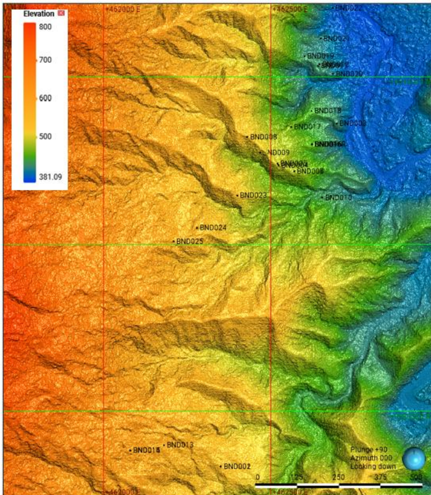
Figure 4.4 – North Bermol DTM Topography
