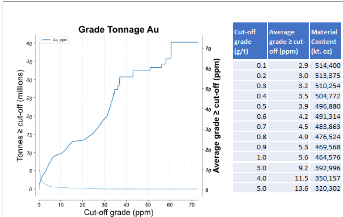
Figure 6.13 – North Bermol Prospect Gold Grade/Tonnage Curve
