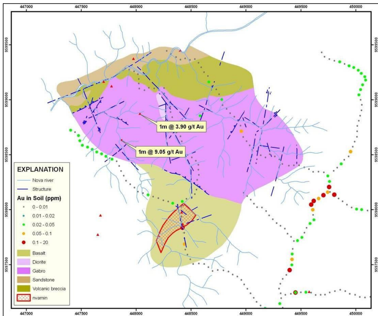
Figure 2.26 – Nova Prospect Geology and Summary Assays
