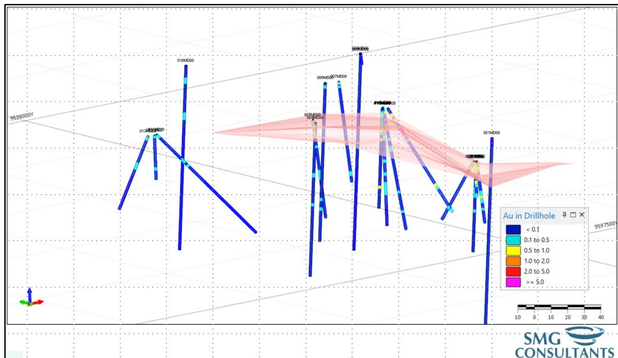
Figure 2.21 – Oblique View Boreholes and Mineralisation Wireframe Mafi
