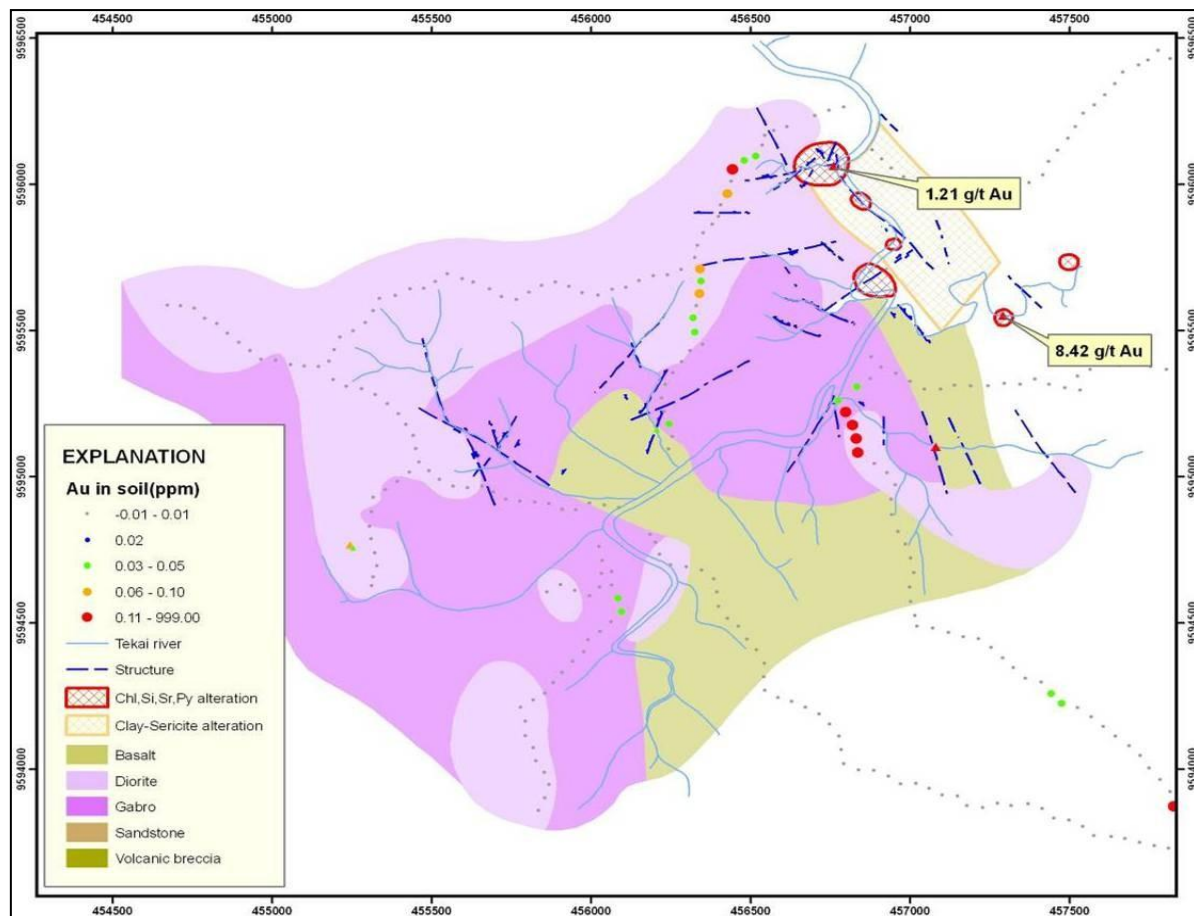
Figure 2.27 – Tekai Prospect Geology
