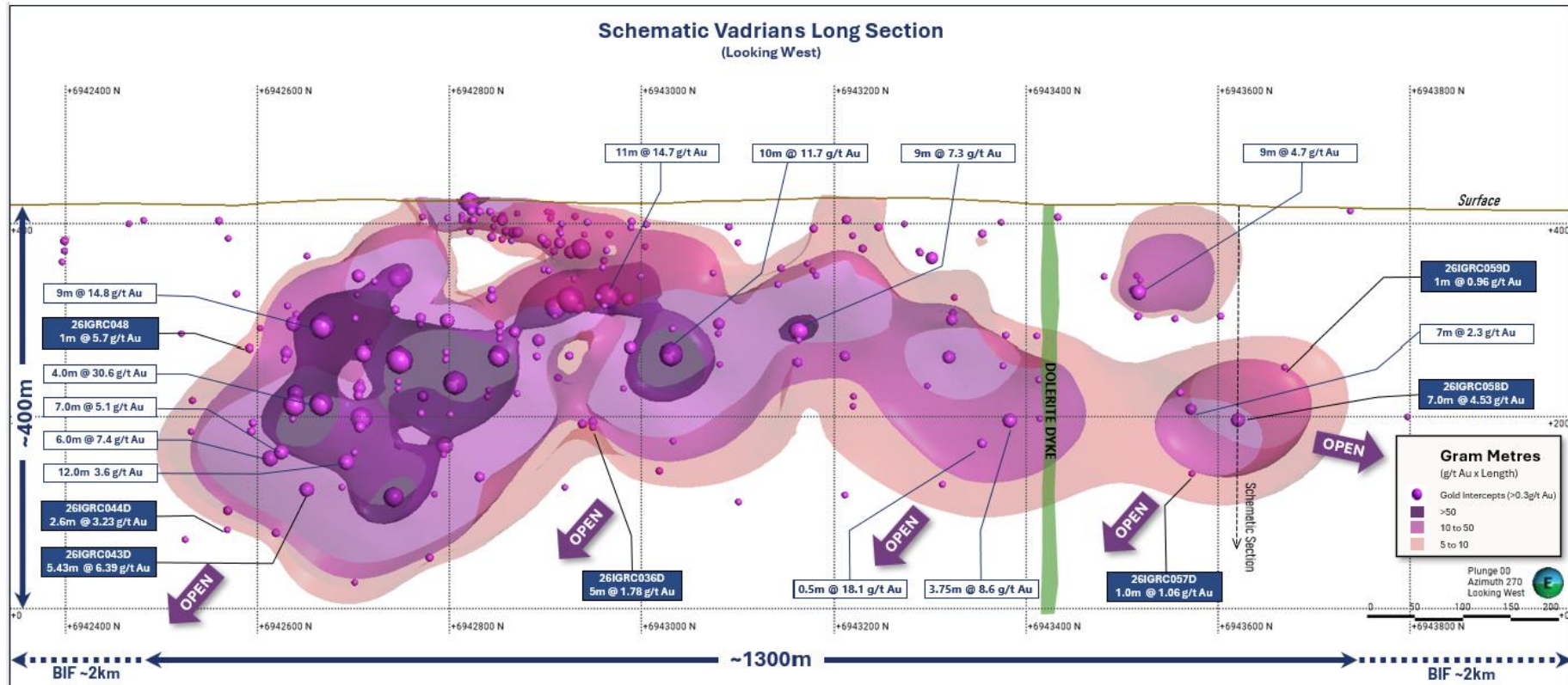
Figure 2: Schematic long section of the Vadrians gold deposit showing significant new drill intersections (blue boxes) with gram-metre contour interpretation and extrapolation for exploration search areas. Note growing gold mineralisation north of the cross-cutting, post-mineralisation dolerite dyke (green).
