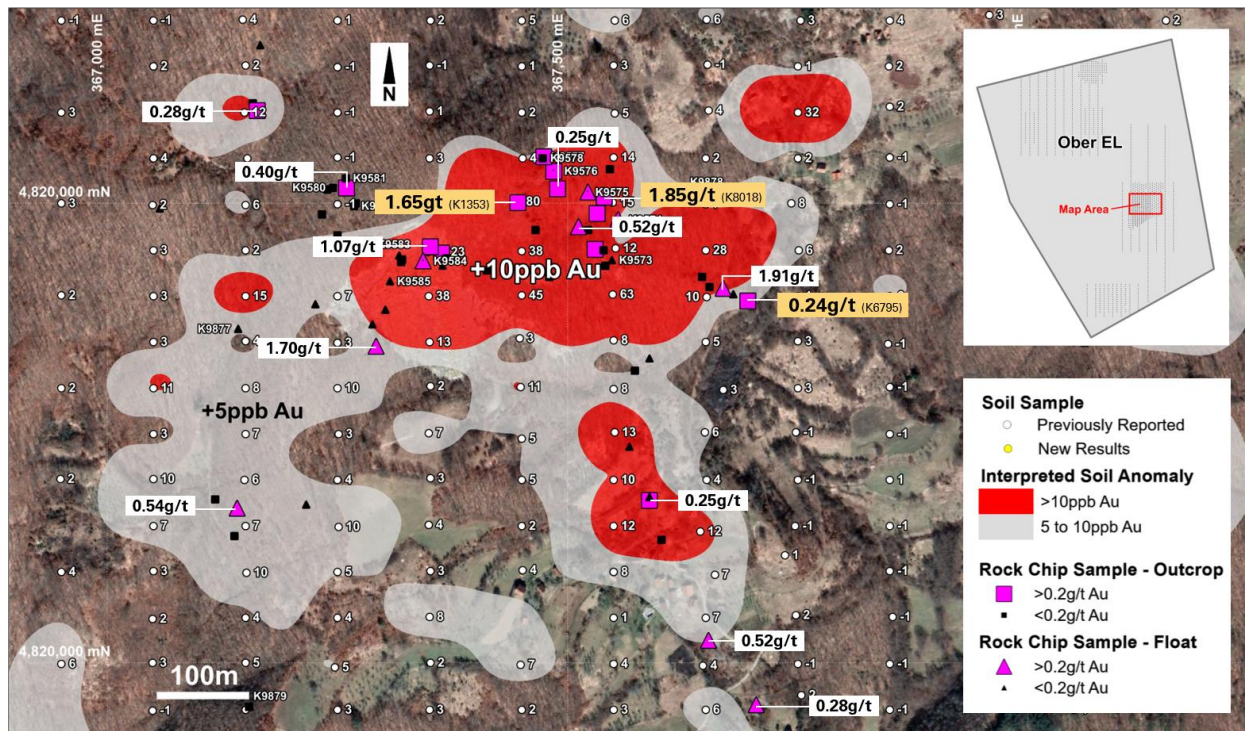
Figure 2: Soil sample results in the Zabrnjica area showing the zone of interpreted +10ppb gold-in-soil anomalism and rock chip sample results.
