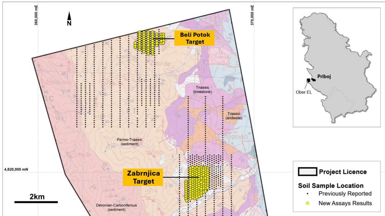
Figure 1: Ober licence area showing location of new soil sample results and Government 1:100K geology map.
