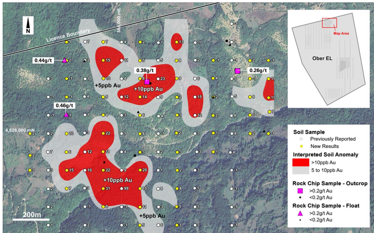
Figure 4: Soil sample results in the Beli Potok area showing the zone of interpreted +10ppb gold-in-soil anomalism and rock chip sample results.
