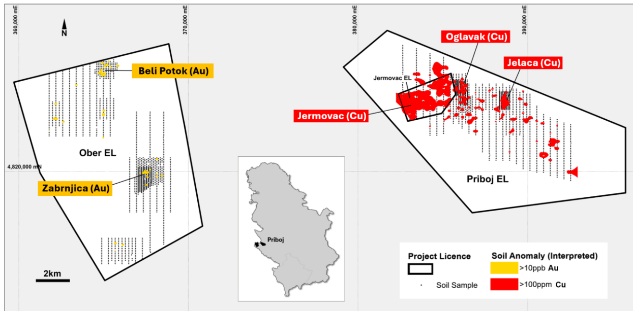
Figure 5: Priboj Project area licences showing priority targets and significant gold and copper soil anomalies.
