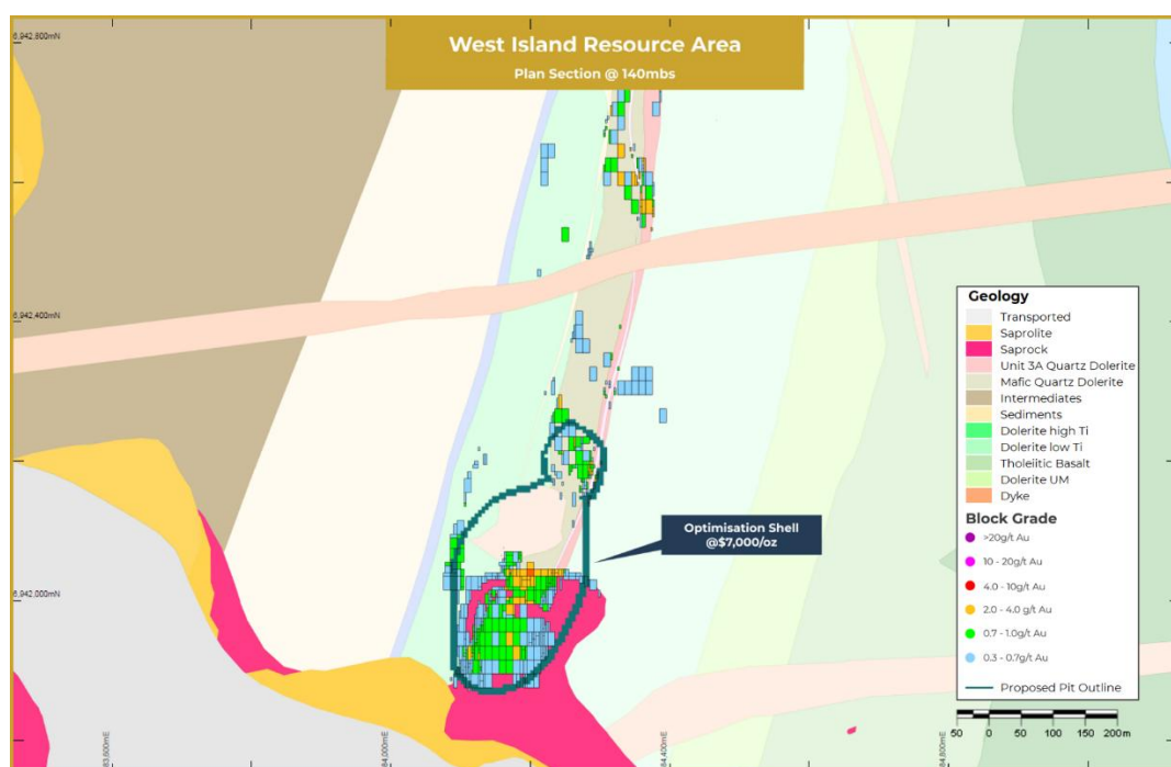
Figure 20: Plan view section of West Island basement geology (transported cover and oxides removed)
