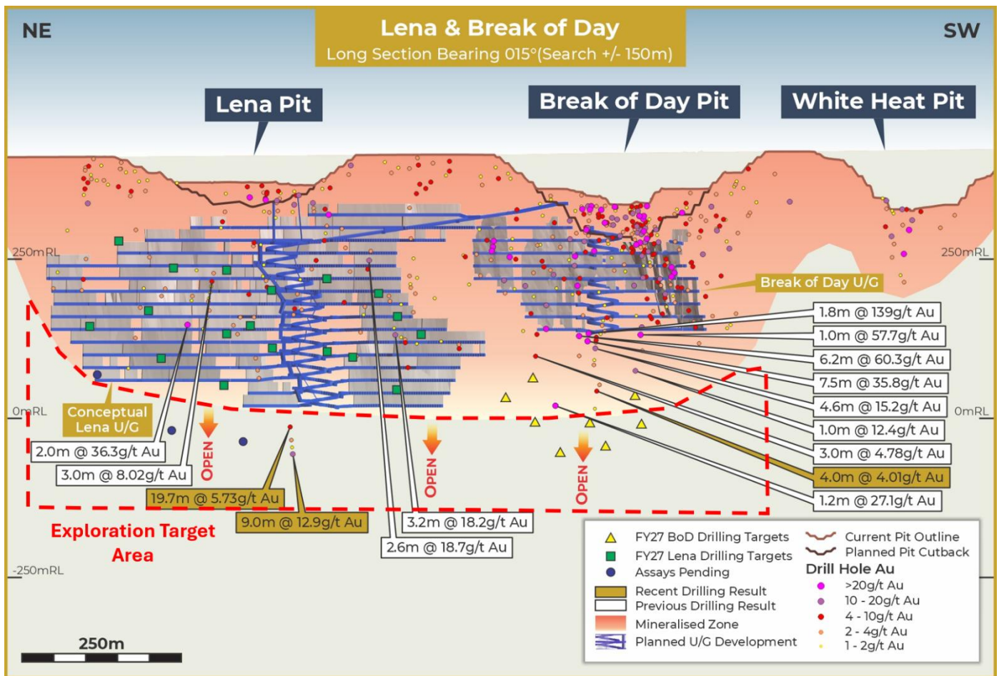
Figure 16: Lena-Break of Day long section with conceptual Lena underground and Exploration Target
