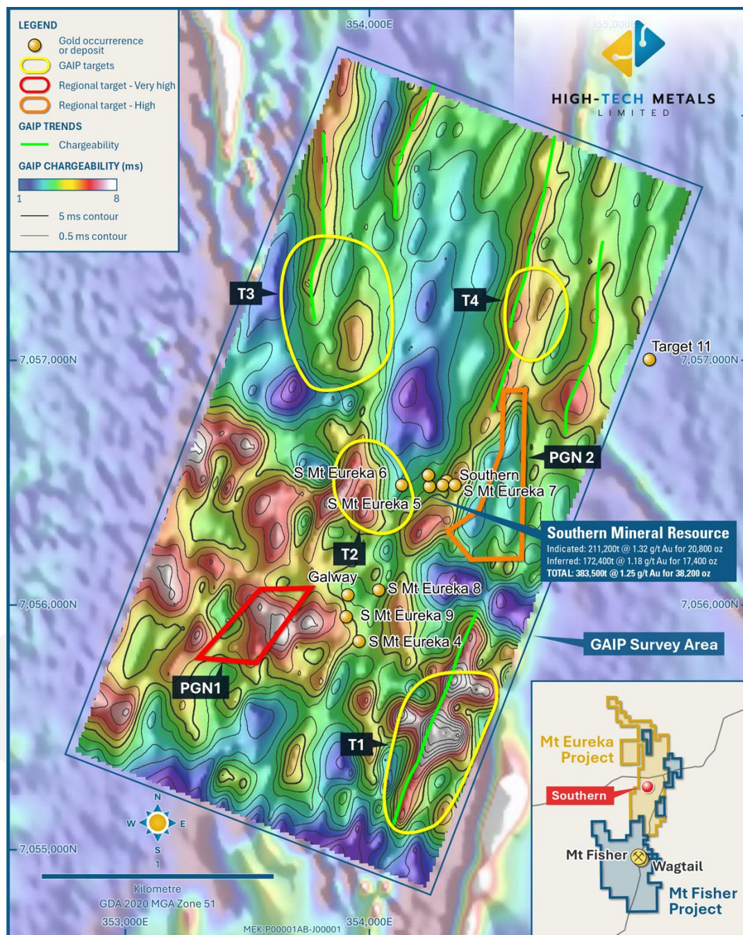
Figure 1: GAIP survey chargeability image with interpreted target areas T1-T4.
