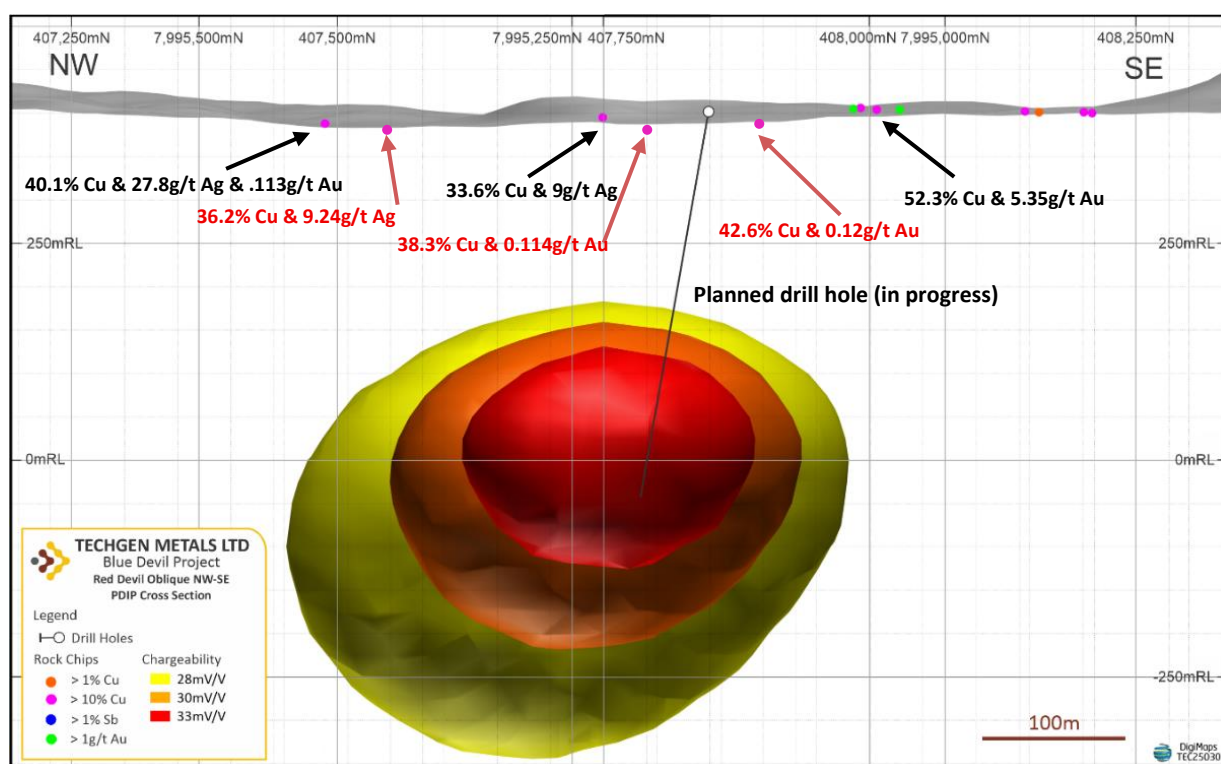
Figure 1: Red Devil 3D IP inversion model with new surface rock chips shown in red and historic in black. Planned drill hole trace.
