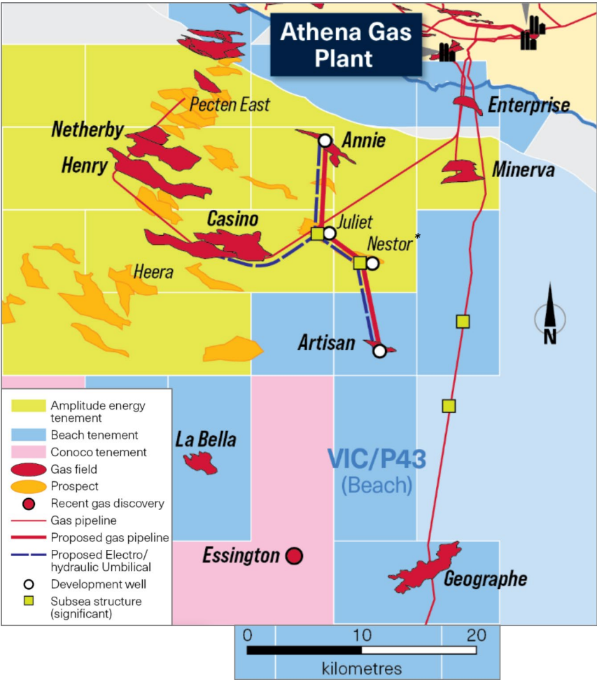
Figure 1: Offshore Otway Basin wells
