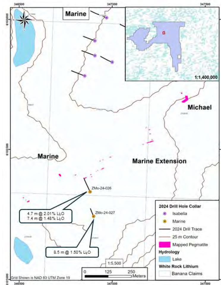
Figure 3-23 2024 drill hole locations at Marine prospect with select results highlighted (source: WhiteRock)
