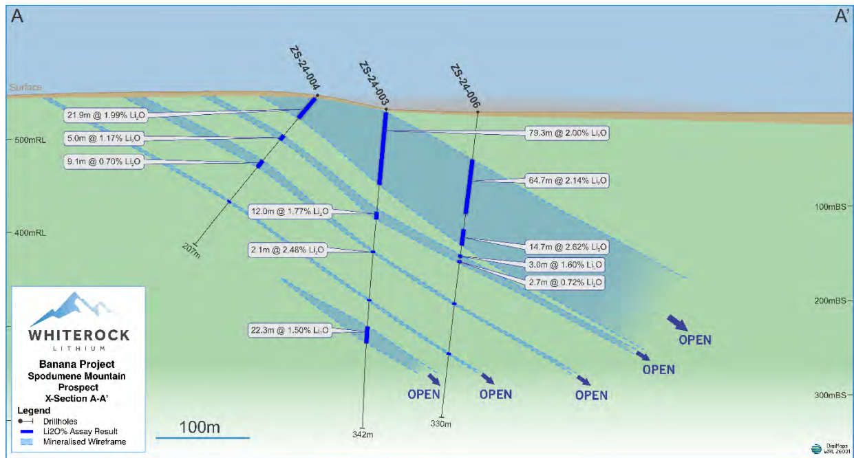
Figure 3-29 Exploration Target cross section A-A' at Spodumene Mountain showing modelled pegmatite dykes (blue) and drill holes with Li 2 O% grades
