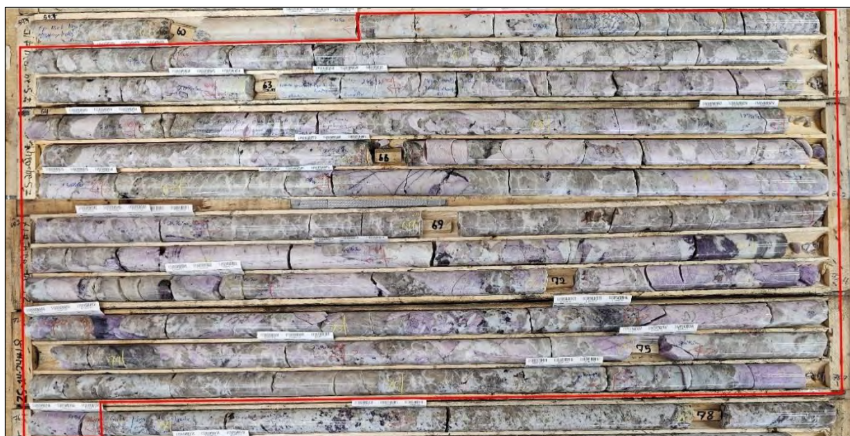
Figure 3-19 Spodumene pegmatite drill core (red box), with 16.2 m at 2.98% \text{Li}_2\text{O} and 352 ppm \text{Ta}_2\text{O}_5 (60.7 to 76.9 m; drill hole ZS-24-024) (source: Dahrouge Geological Consulting, 2025)
