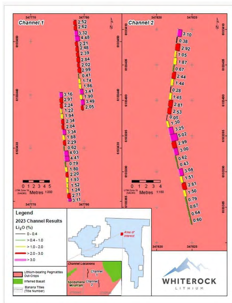
Figure 3-11 Channel sampling #1 and #2 on Spodumene Mountain (source: GMY Consulting, 2024)
