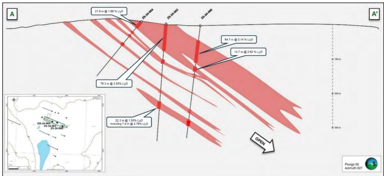
Figure 3-18 Cross-section A-A' Spodumene Mountain pegmatite cluster with select results highlighted. Section location inset (source: Dahrouge Geological Consulting, 2025)
