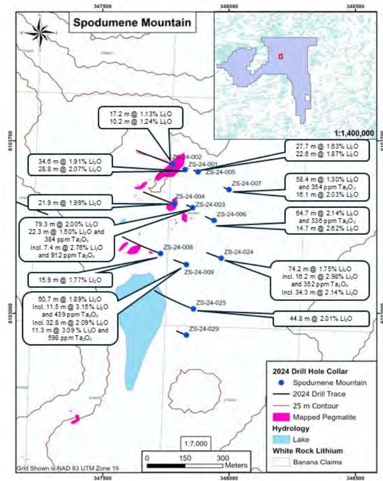
Figure 3-17 Spodumene Mountain 2024 drill hole locations with select results highlighted (source: WhiteRock)
