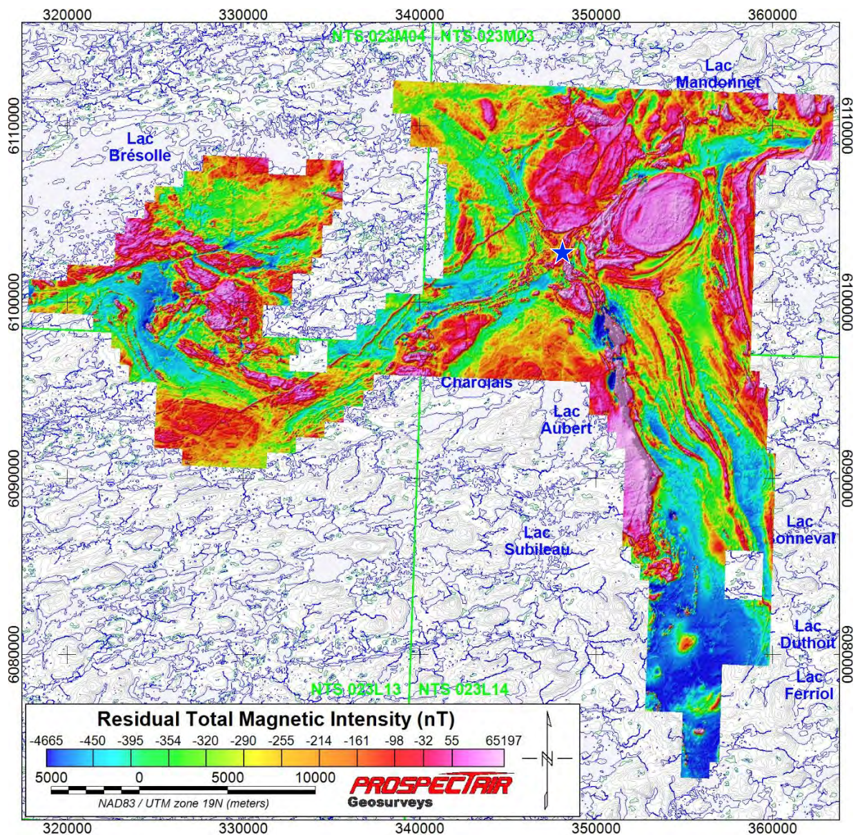
Figure 3-27 Residual Total Magnetic Intensity with equal area colour distribution. Blue star shows the location of the Banana Lithium Project (Source: Dynamic Discovery Geoscience, 2025)
