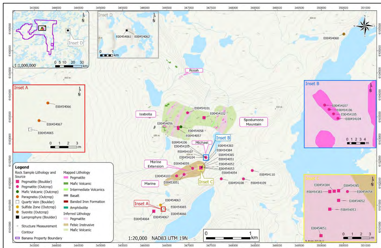
Figure 3-14 Location map for the 2024 rock sample \text{Li}_2\text{O}\% results (source: Dahrouge Geological Consulting, 2025)
