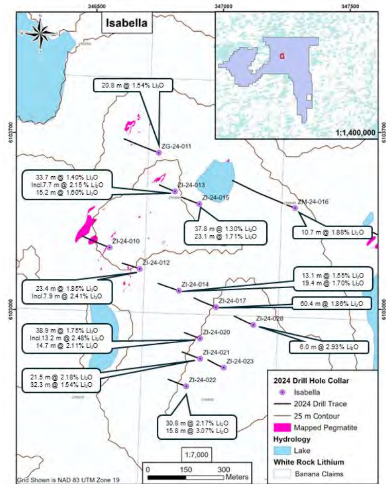
Figure 3-20 2024 drill hole locations at Isabella prospect with select results highlighted (source: WhiteRock)
