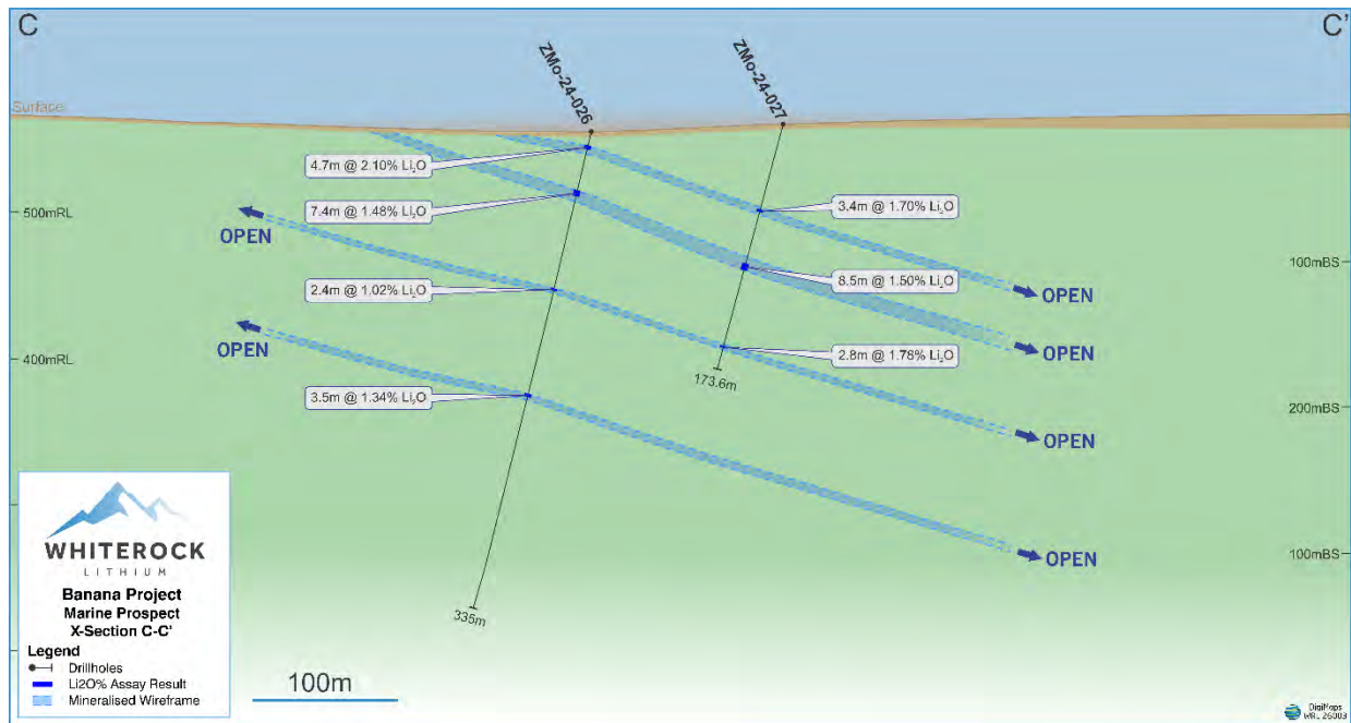
Figure 3-31 Exploration Target cross section C-C' at Marine showing modelled pegmatite dykes (blue) and drill holes with \text{Li}_2\text{O}\% grades
