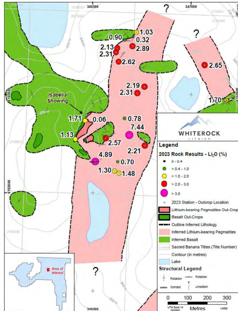
Figure 3-13 Grab sample locations and Li 2 O grades for Isabella area (source: WhiteRock, 2024)
