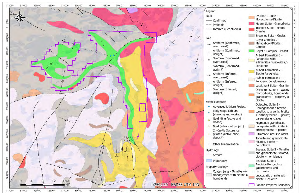
Figure 3-6 Project Geology Map (modified after: Dahrouge Geological Consulting, 2025)
