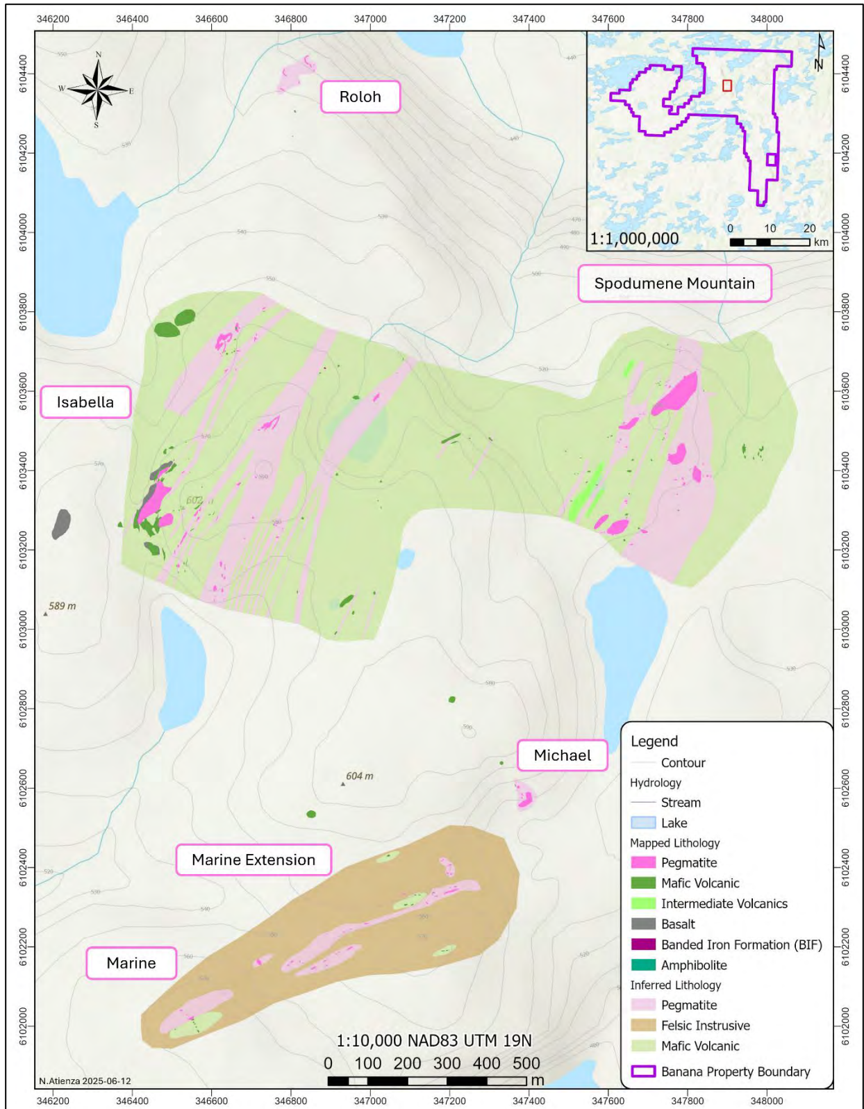
Figure 3-8 Geological map of the Project showing the spodumene-bearing pegmatite clusters (source: Dahrouge Geological Consulting, 2025)
