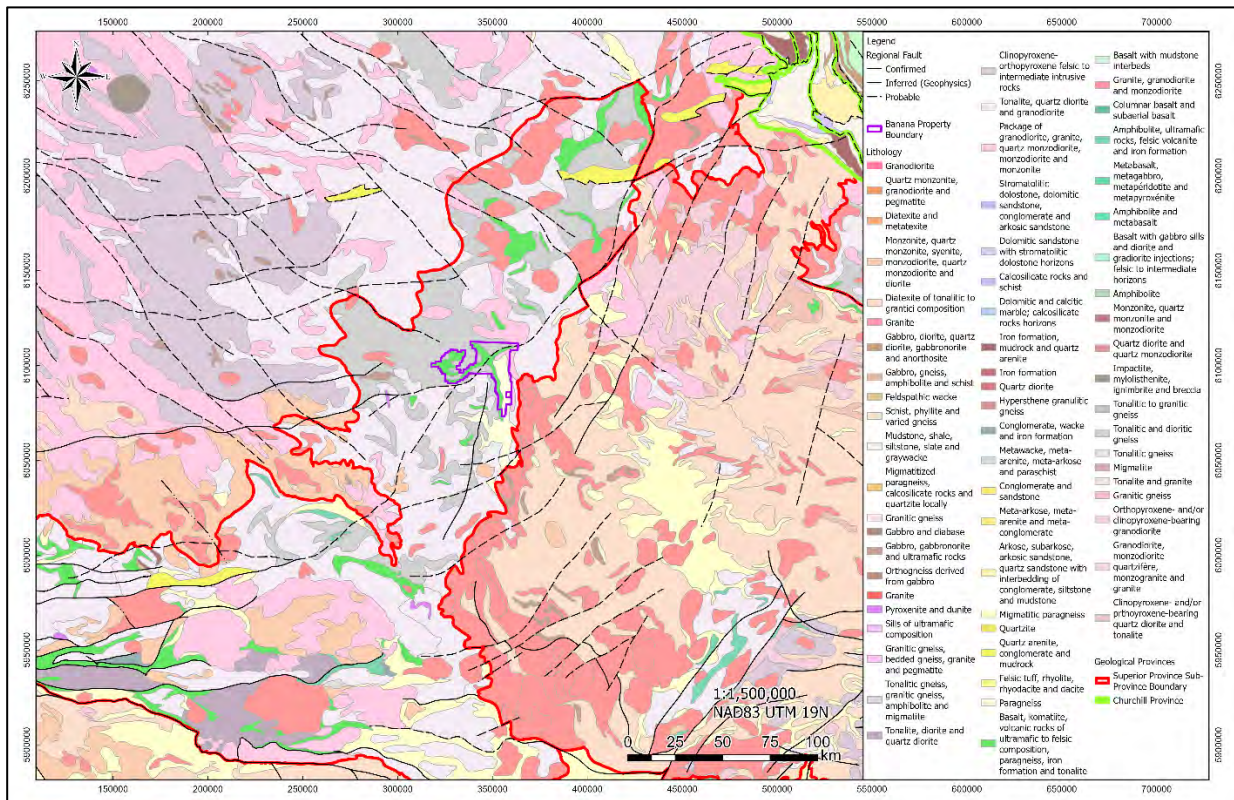
Figure 3-5 Regional geological setting with the Banana Lithium Project area (modified after: Dahrouge Geological Consulting, 2025)
