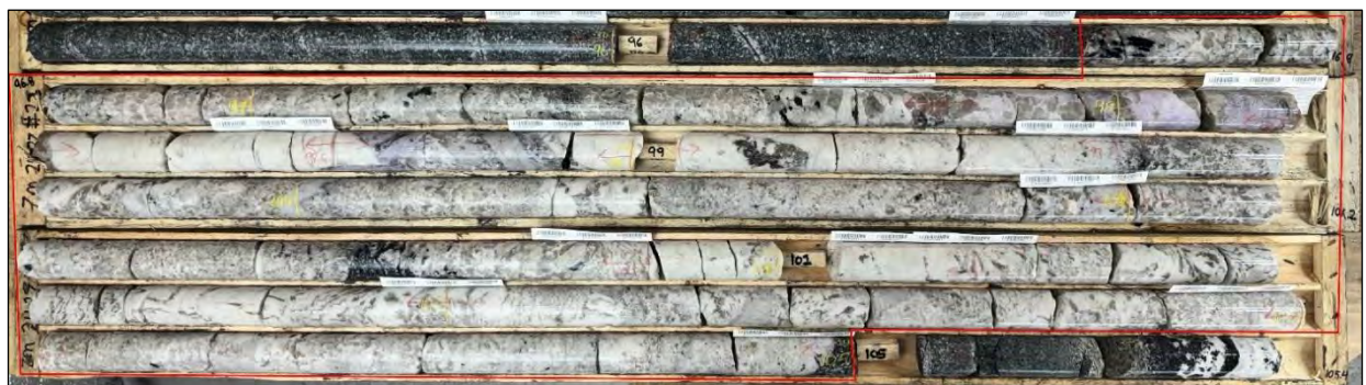
Figure 3-24 Spodumene pegmatite drill core (red box), grading 1.50% \text{Li}_2\text{O} and 165 ppm \text{Ta}_2\text{O}_5 over 8.5 m (96.5 to 105.5 m; drill hole ZMo-24-027) (source: Dahrouge Geological Consulting, 2025)
