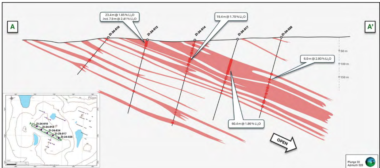
Figure 3-21 Cross-section A-A' Isabella pegmatite cluster with select results highlighted. Section location inset (source: Dahrouge Geological Consulting, 2025)
