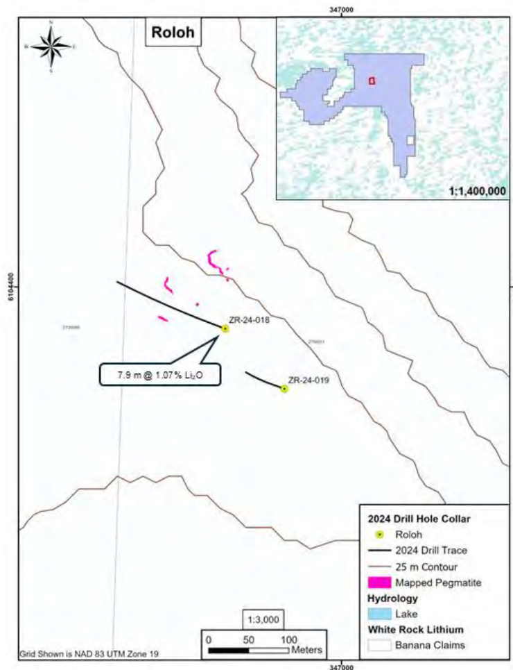
Figure 3-25 2024 drill hole locations at Roloh prospect with select results highlighted (source: WhiteRock)
