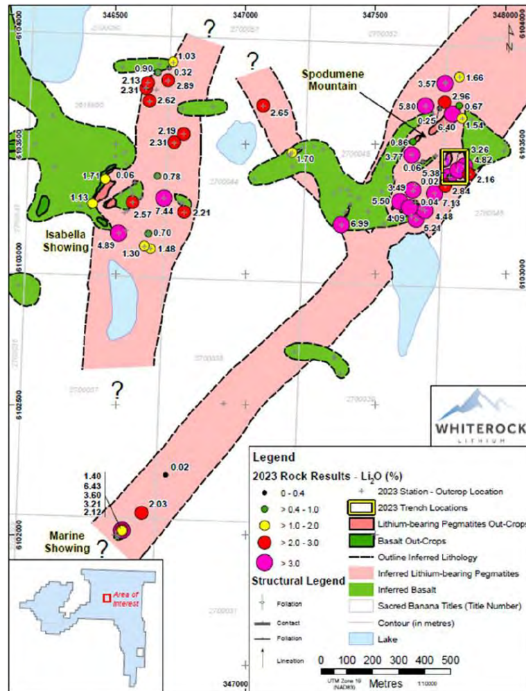
Figure 3-12 Grab sample locations and Li 2 O grades for Spodumene Mountain, Isabella and Marine areas (source: GMY Consulting, 2024)
