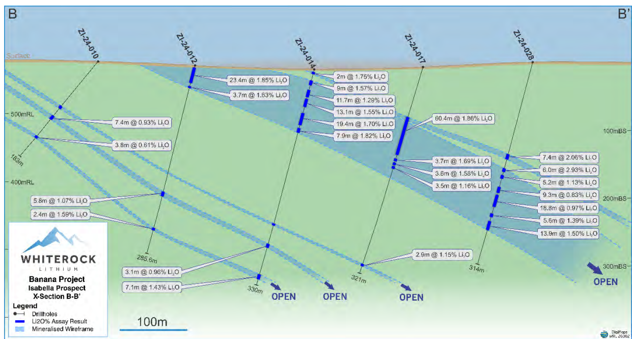
Figure 3-30 Exploration Target cross section B-B' at Isabella showing modelled pegmatite dykes (blue) and drill holes with Li 2 O% grades
