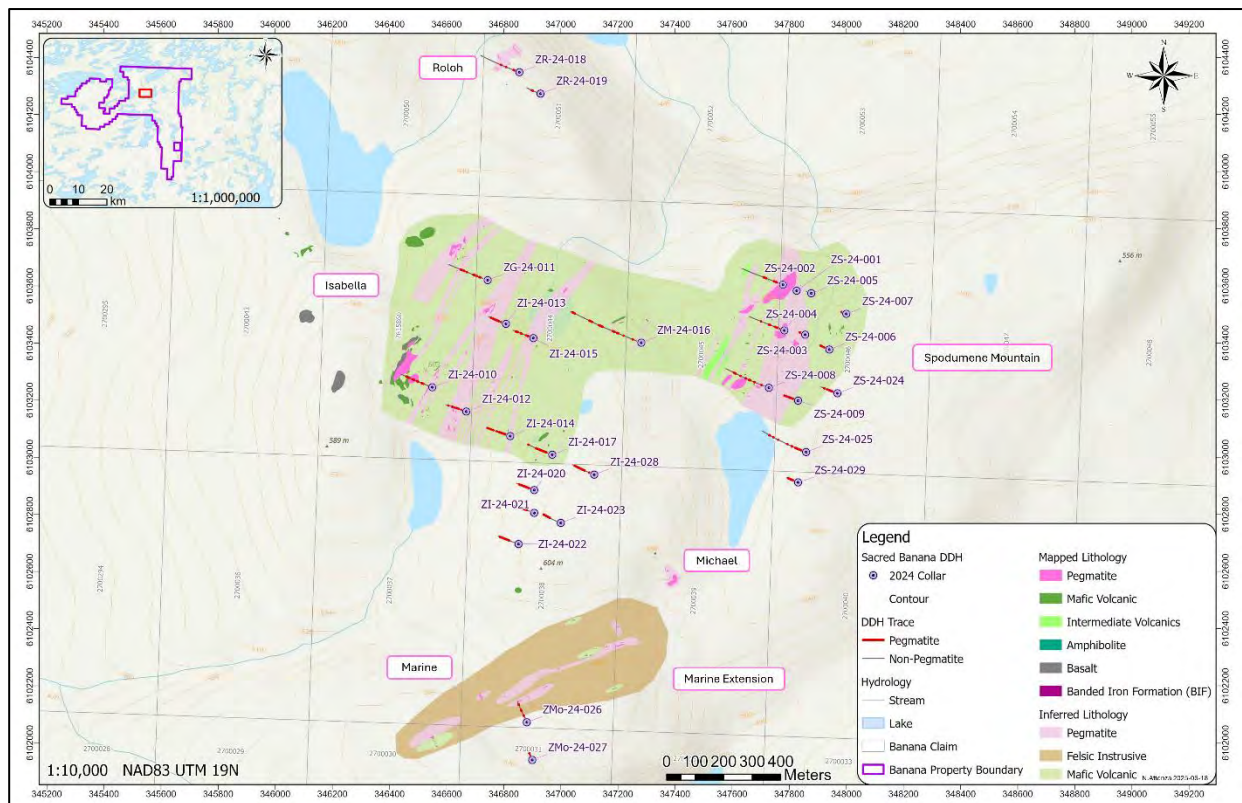
Figure 3-16 Map of 2024 drill holes (source: Dahrouge Geological Consulting, 2025)
