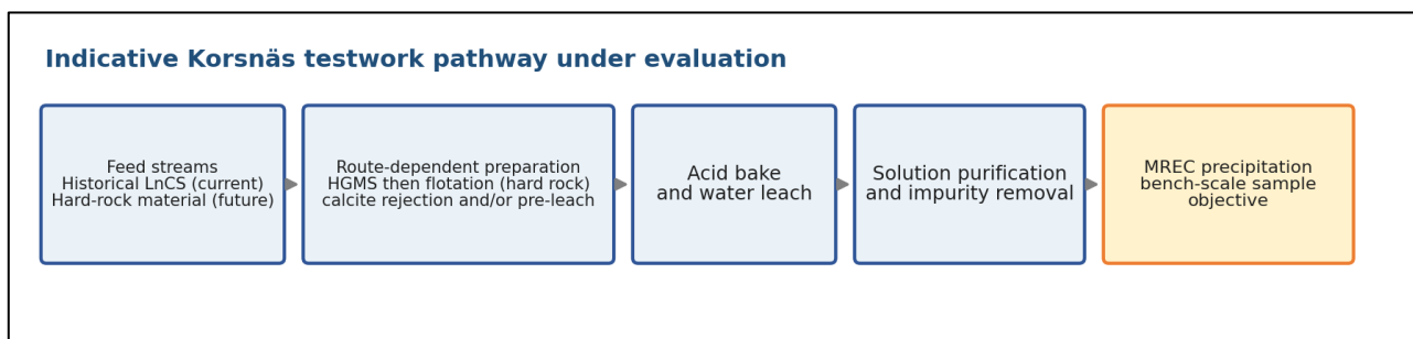
Figure 3: Indicative Korsnäs testwork pathway under evaluation. The sequence and unit operations may change as test work progresses.
