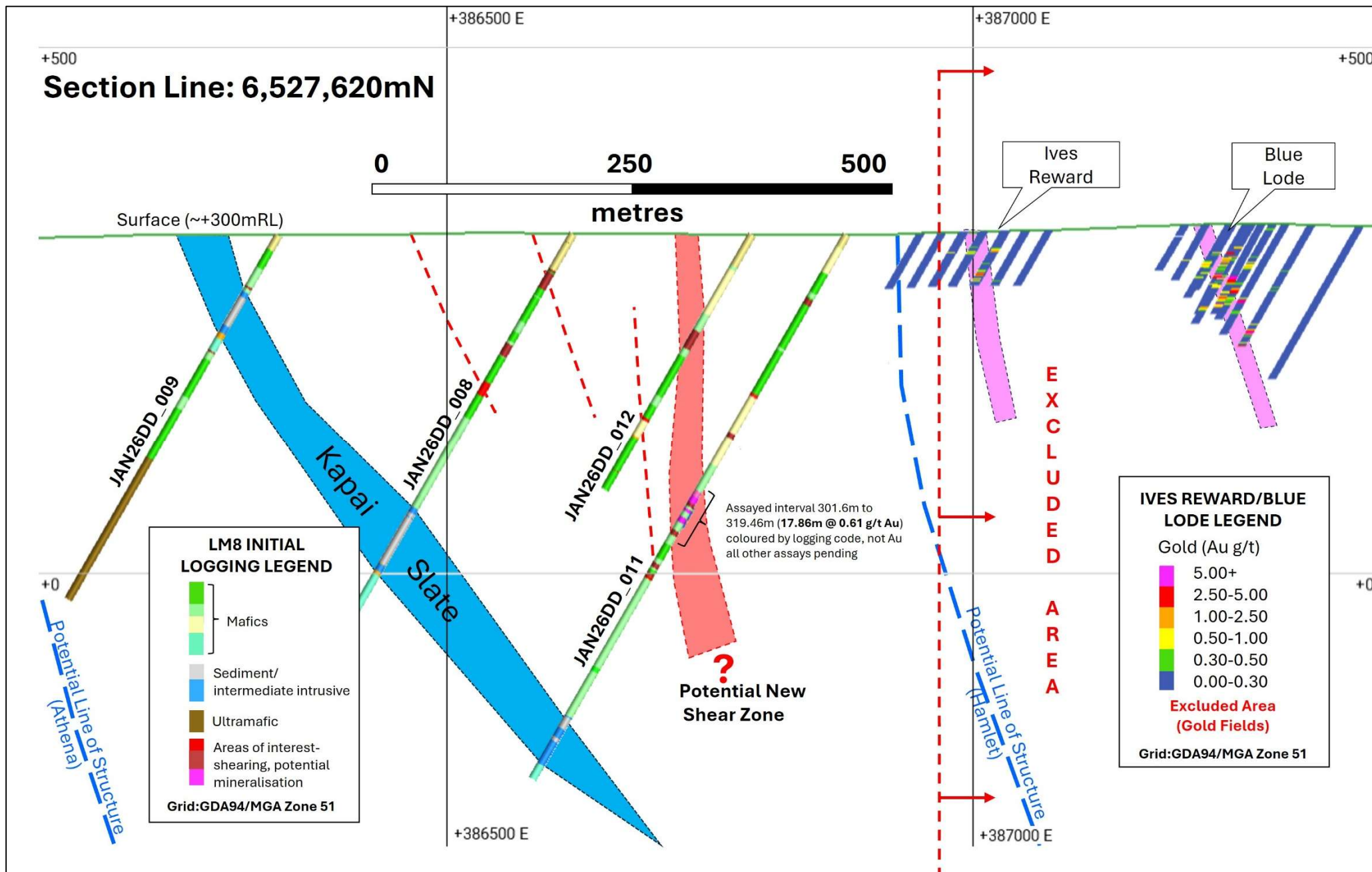
Figure 3: Cross-sectional view of preliminary interpretation of structure, lithology and potential gold mineralisation – 6,527,620mN
