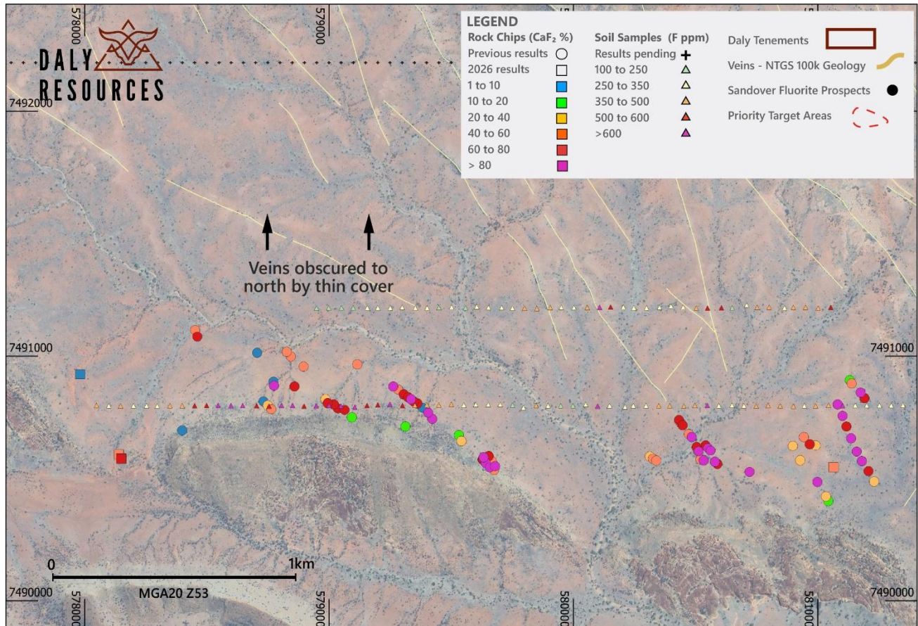
Figure 2: Map showing new rock chip and first-pass soil assay results at the western end of the soil lines, where a ~1km wide zone of strongly anomalous \text{CaF}_2 was returned from the soils. Follow-up investigation has found further structures which had not previously been identified.
