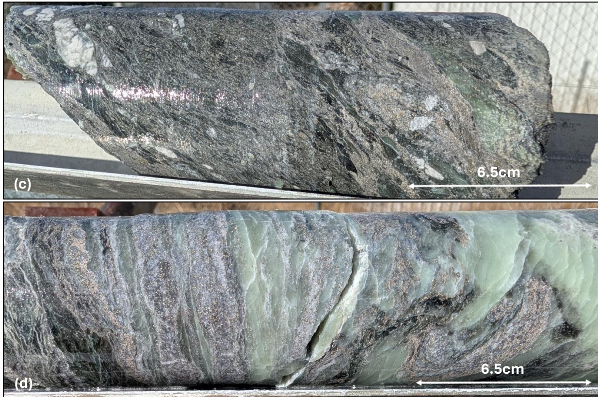
Figure 1. (a) Massive sphalerite-pyrite-galena-chalcopryrite mineralisation hosted within a talc shear zone in BLRCDD005, 251.75m. (b) Heavy disseminated sphalerite-pyrite-galena-chalcopryrite mineralisation in BLRCDD004, 212.5m. (c) Semi-massive sphalerite-pyrite-galena in talc-rich shear zone in BLRCDD005, 247m. (d) Sphalerite-galena-pyrite mineralisation in talc-rich shear zone in BLRCDD005, 251.4m. Visual estimate only; assays pending. Refer to Table 2 for visual sulphide estimates and cautionary statement.
