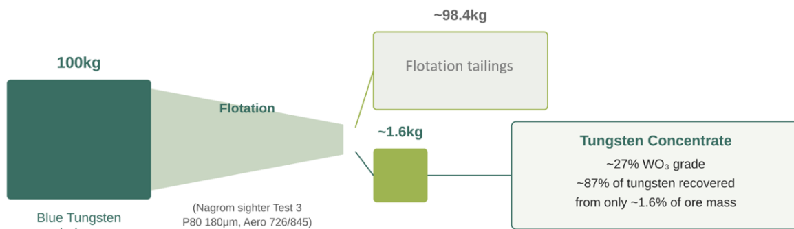
Figure 2: Illustrative mass balance for Test 3, based on Nagrom sighter flotation results. Indicative only; not a final product specification.
