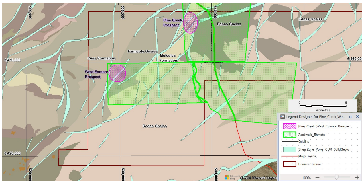
Figure 2: Enmore Solid Geology and Prospects
