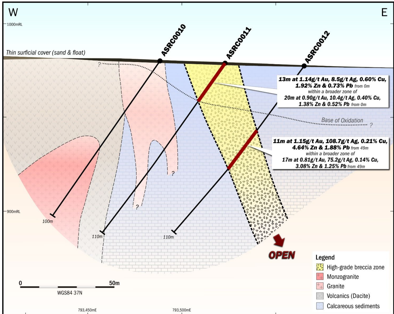
Figure 3. Cross section 2679060mN through the new polymetallic breccia discovery showing shallow high-grade mineralisation open at depth. East-west section through ASRC0010, ASRC0011 and ASRC0012 showing the interpreted Au-Ag-Cu-Pb-Zn-rich breccia beneath thin surficial cover. The breccia remains open at depth, with true width and overall geometry yet to be established.
