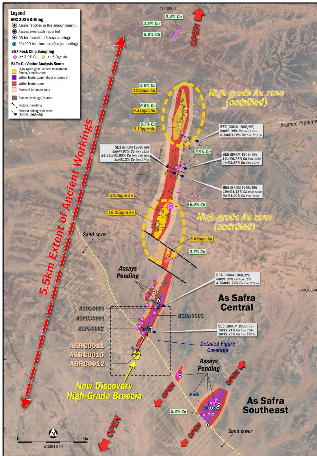
Figure 1. As Safra mineralised corridor highlighting the new high-grade polymetallic breccia discovery and extensive ancient workings. Plan view showing the 5.5 km mineralised corridor, SNX high-grade Cu and Au rock samples, drilling and Bi-Te-Cu geochemical vectoring. The new Au-Ag-Cu-Pb-Zn-rich breccia lies beneath shallow cover approximately 400 m south of the Central Zone and remains open along strike and at depth.
