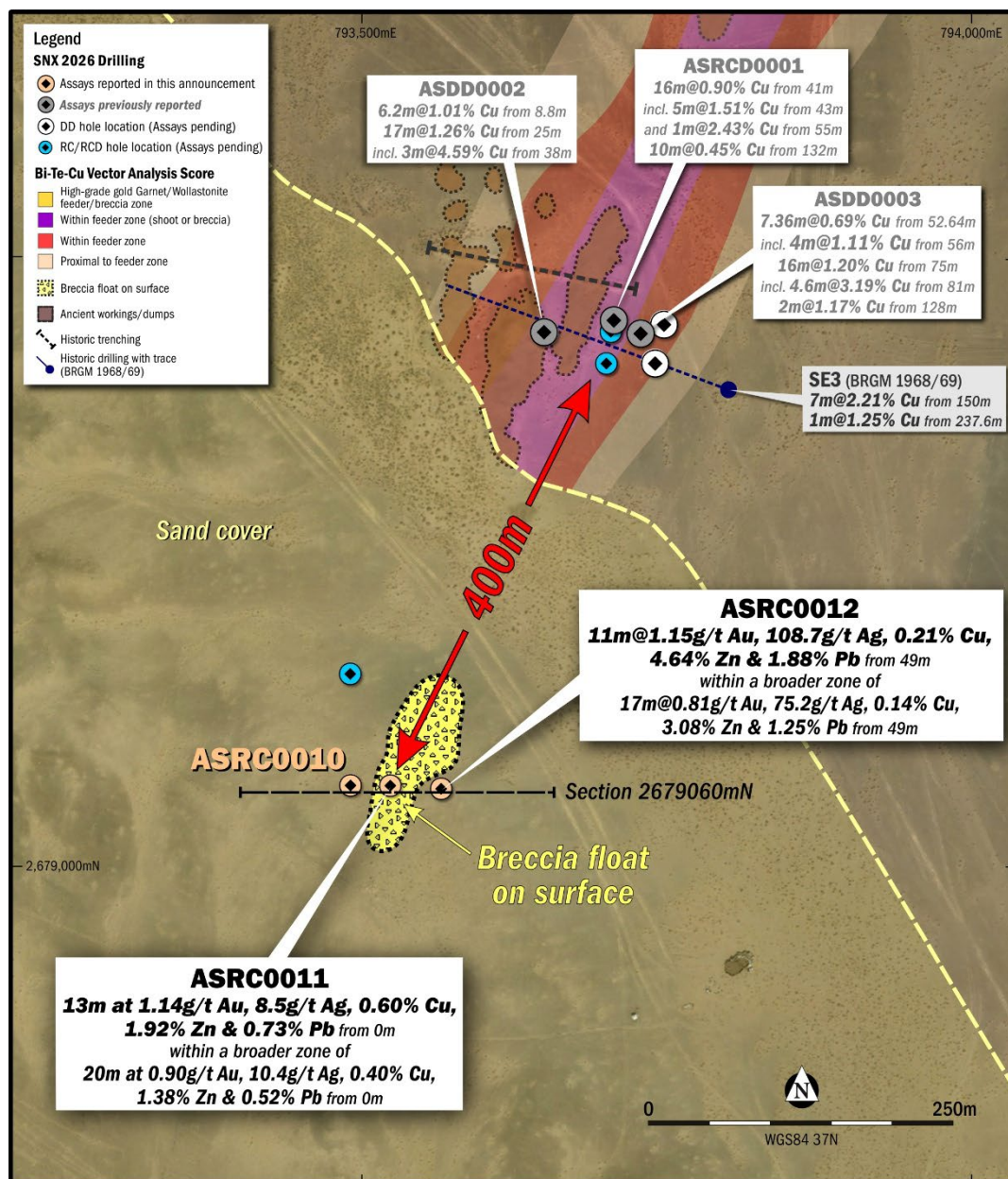
Figure 2. Detailed plan of the new polymetallic breccia discovery, approximately 400 m south of the Central Zone. High-grade Au-Ag-Cu-Pb-Zn mineralisation was intersected in RC holes ASRC0011 and ASRC0012 beneath shallow sand cover, adjacent to breccia float at surface. The discovery remains open along strike and at depth. Section 2679060mN is shown in Figure 3.
