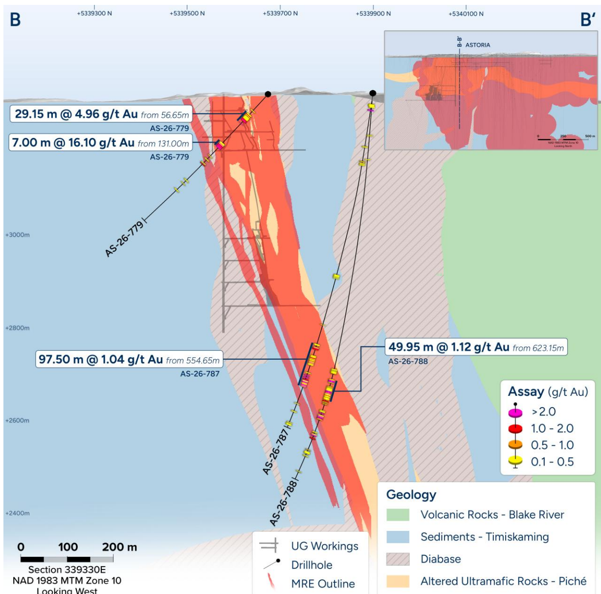
Figure 3 – Astoria long section showing drilling and current MRE outline.
