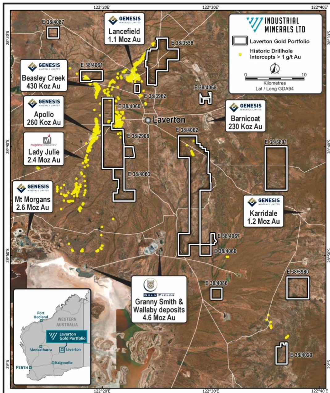
Figure 1: Laverton gold region, IND tenements, existing reported resources and historic > 1 g/t Au drill intercepts
