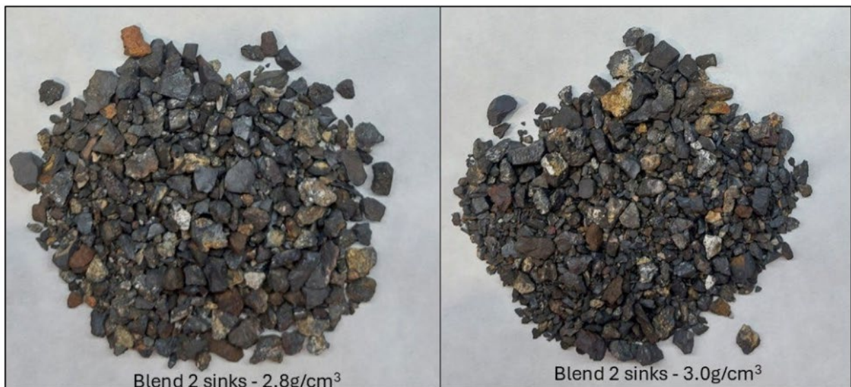
Figure 4. Blend 2 sinks at 2.8g/cm 3 and 3.0g/cm 3 with grades of 41.1% and 43.8% Mn respectively. Pile width is about 15cm.
