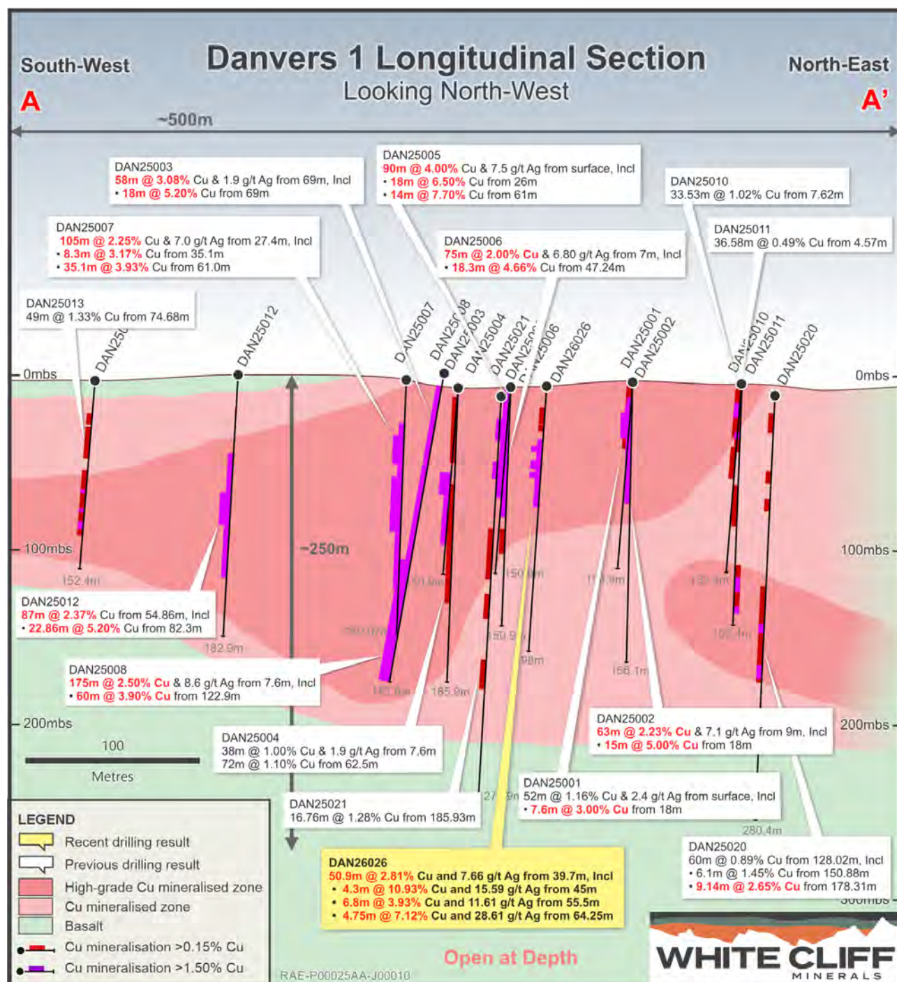
Figure 2 - Long section of Danvers 1, with the Company's first diamond drill hole DAN26026 highlighted.
