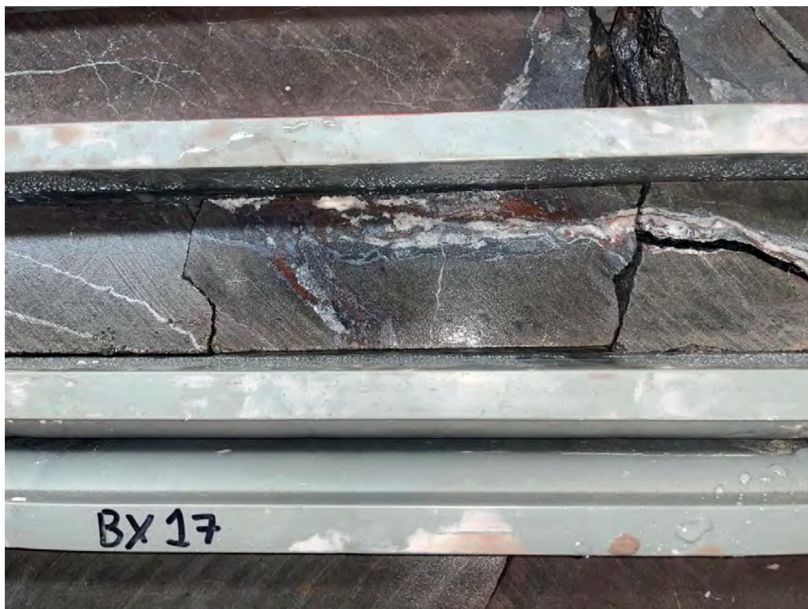
Figure 4 - Photograph of cut NQ2 diameter core containing vein-hosted chalcocite from 66.4m downhole in drillhole DAN26026
