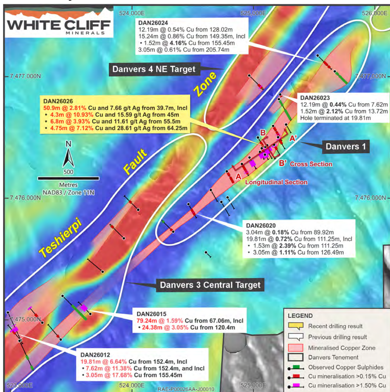
Figure 1 - Map of 2026 RC and diamond drillholes in the Teshierpi Fault Zone. Basemap of EM anomalism (X component) from 2025 geophysical survey. Interpreted mineralisation trend highlighted by white outline between the observed downhole intervals of copper sulphides.
