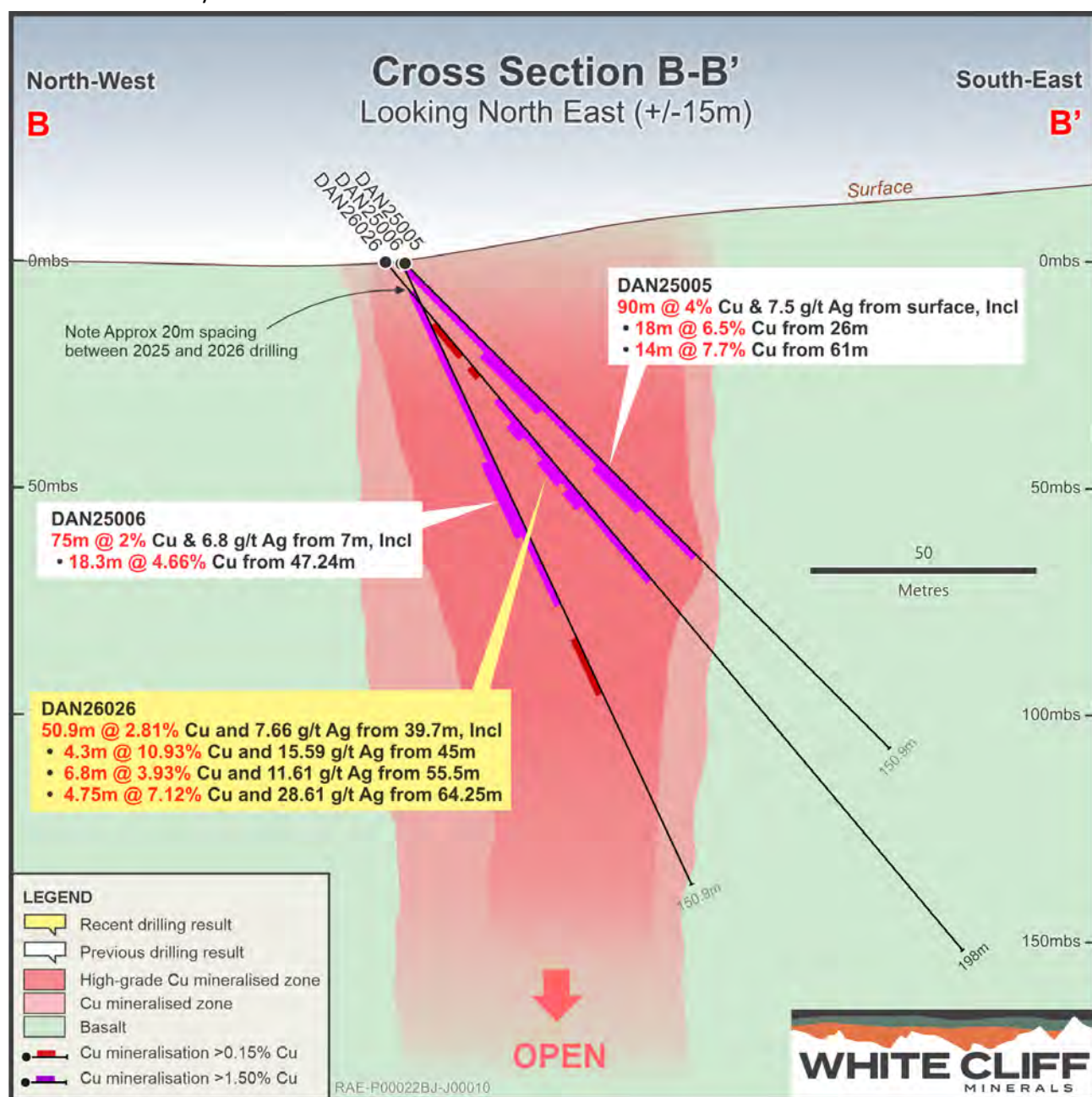
Figure 3 - Cross section of drillhole DAN26026 which is within the Danvers 1 deposit. This was an infill & step out to holes DAN25005 & DAN@5006 that was drilled in 2025 with an RC Rig. DAN26026 is White Cliff's first diamond drillhole into Danvers 1.
