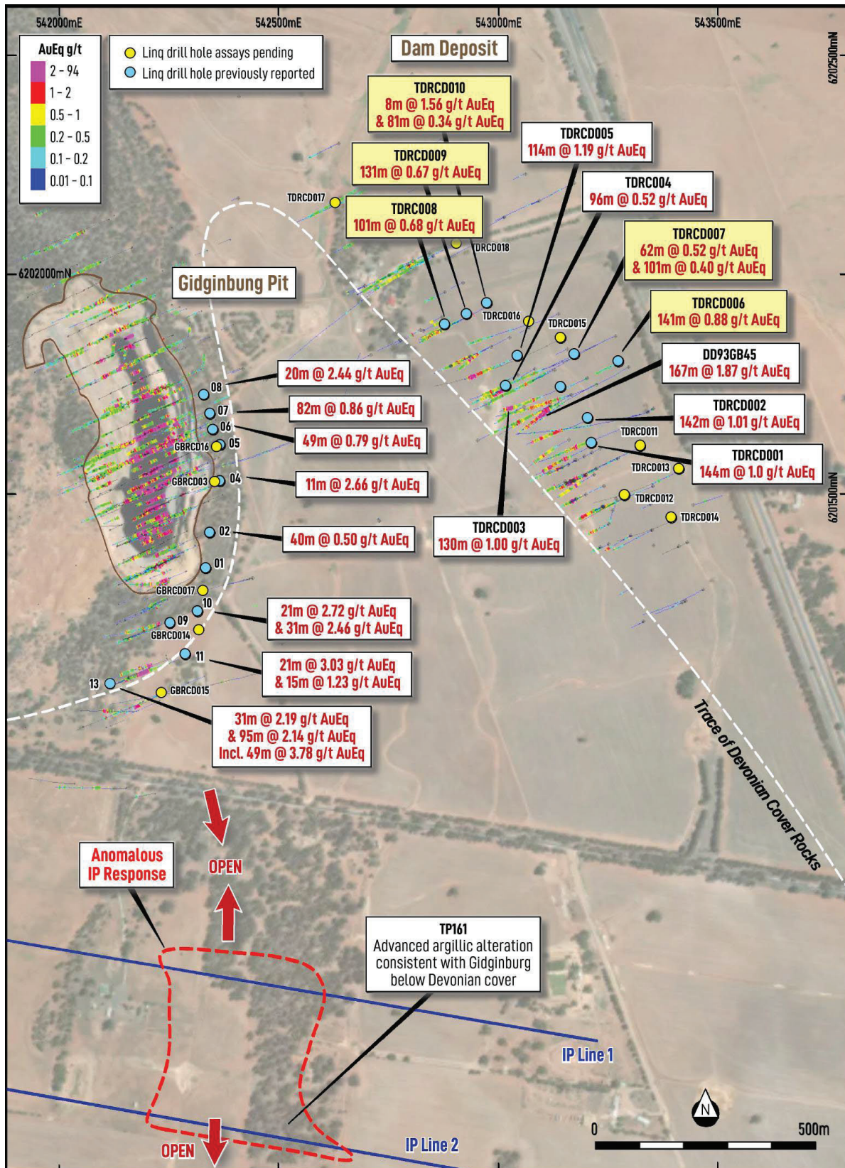
Figure 3: Plan image of Gidginbung and the Dam illustrating the location of the Gidginbung South IP lines and associated anomalous IP response.
