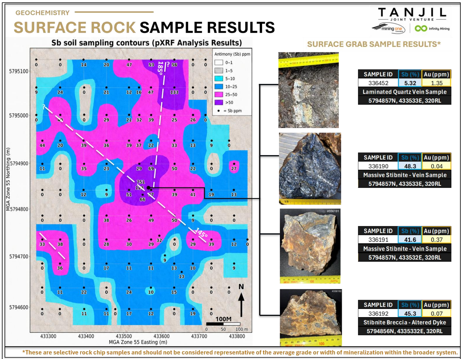
Figure 5: Tanjil Dome 50 m x 50 m Soil Sampling Grid (Sb ppm) with Surface Rock Sample Assays and Locations
