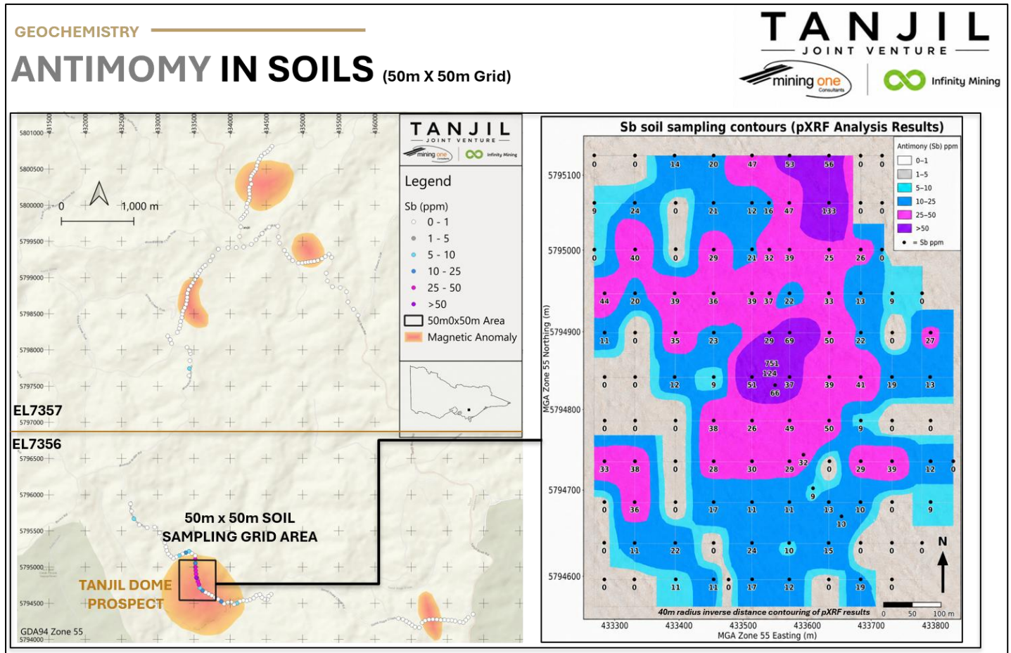
Figure 6: Tanjil Dome Prospect 50 m x 50 m Soil Sampling Results – Antimony ppm (pXRF)
