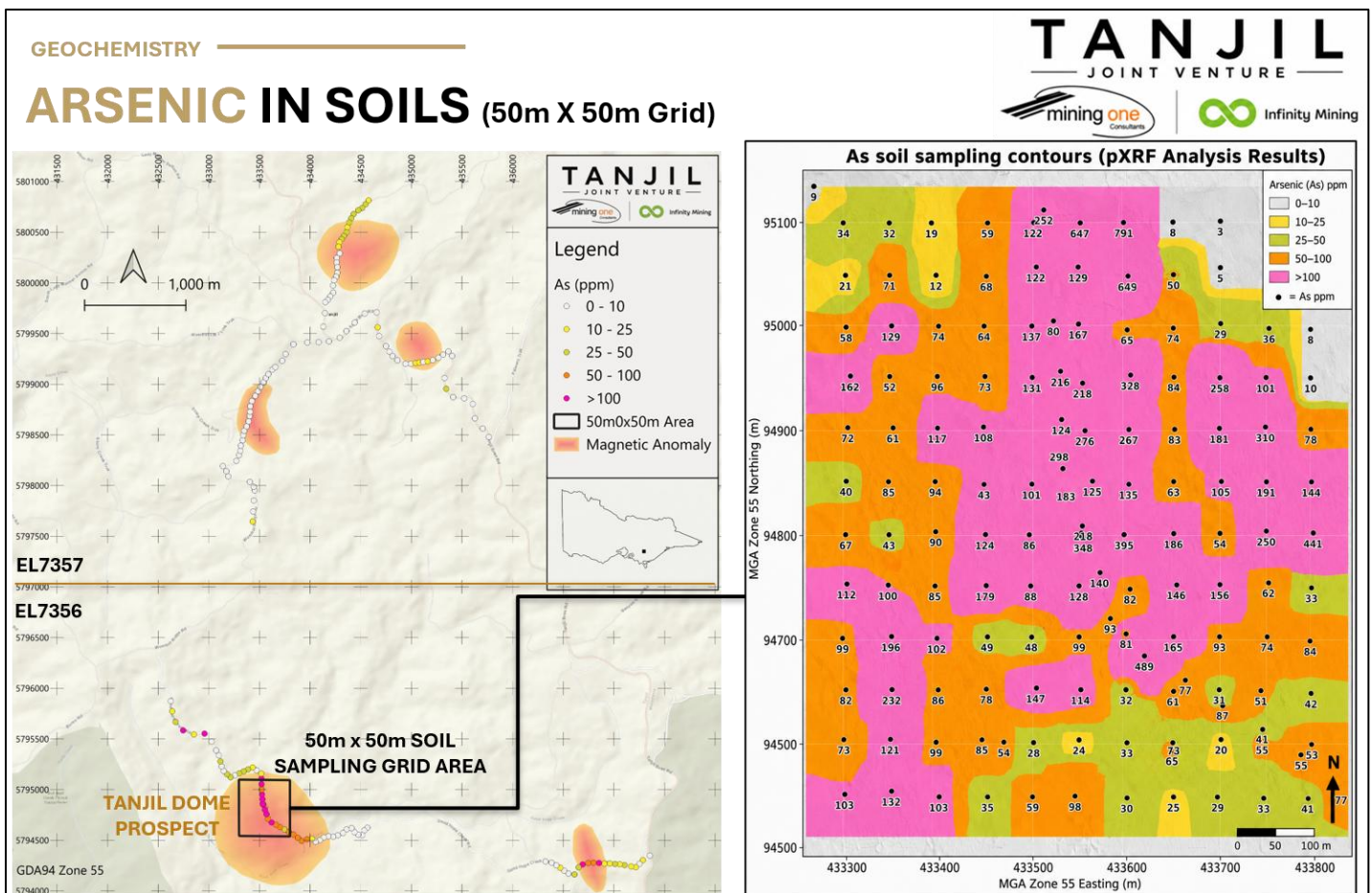
Figure 8: Tanjil Dome Prospect 50 m x 50 m Soil Sampling Results – Arsenic ppm (pXRF)
