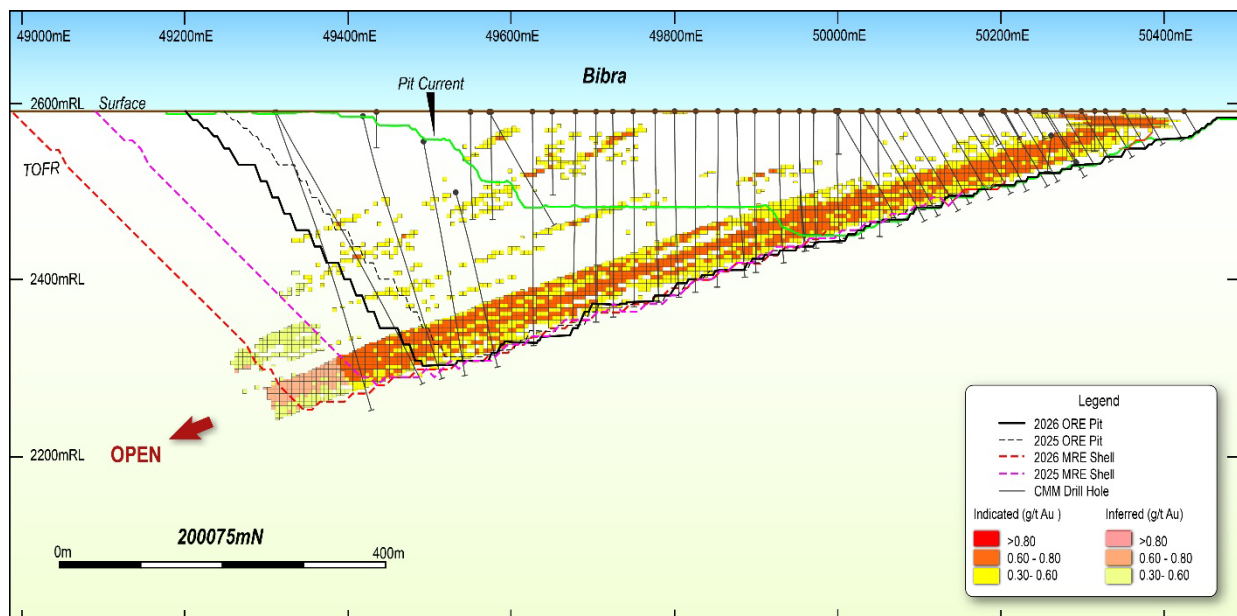
Bibra pit cross section.
