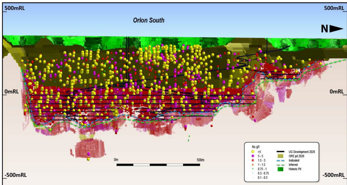
Orion South Underground Mineral Resource – Long Section.
