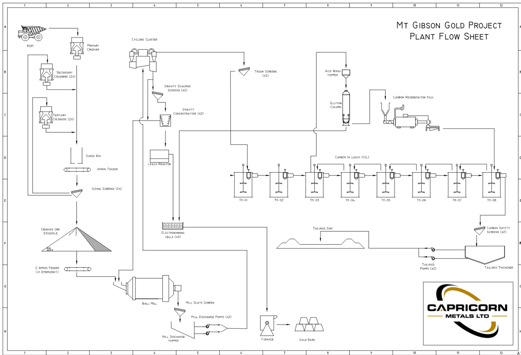
MGGP Processing Plant Flow Sheet.
