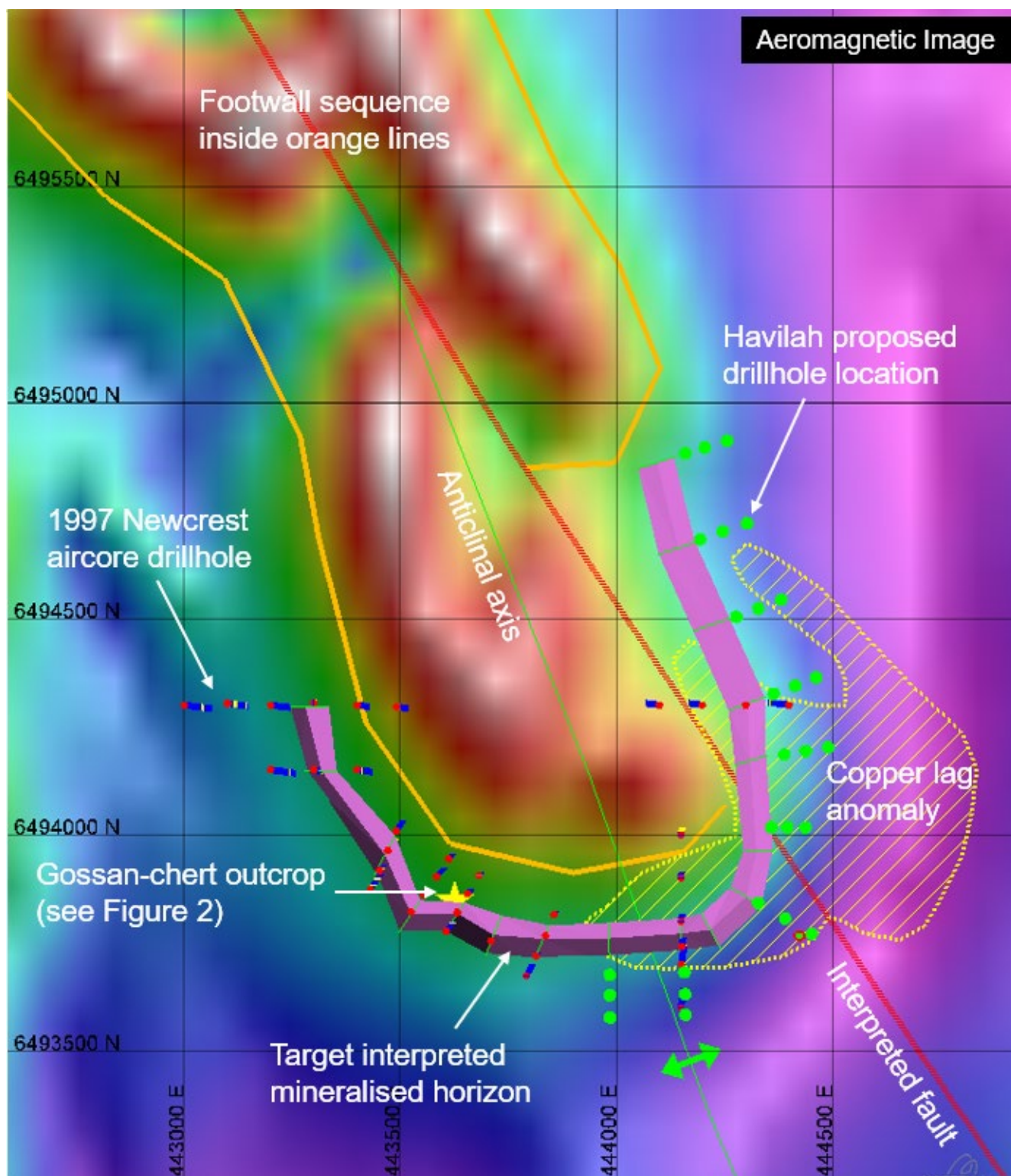
Figure 1 Geological interpretation of the Brooks Dam prospect on aeromagnetic image, showing interpreted magnetic footwall rocks (red colour), the target stratabound ironstone horizon folded around a south-plunging anticline (purple), copper lag geochemical anomaly (yellow striped), previous Newcrest aircore drillholes (red dots are collar locations) and Havilah's planned drillhole collar locations (green dots). The earlier Newcrest aircore drillholes were unsuccessful in penetrating the hard, iron-rich stratabound horizon. The yellow star shows the location of the gossan-chert outcrop expression of the interpreted Kalkaroo stratabound host horizon as shown in Figure 2.
