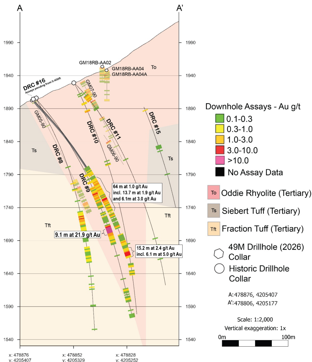
Figure 2: Cross-Section Showing Hole DRC#16
