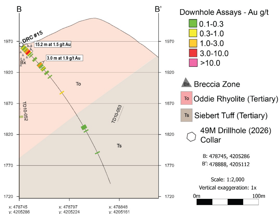
Figure 3: Cross-Section showing Hole DRC#15
