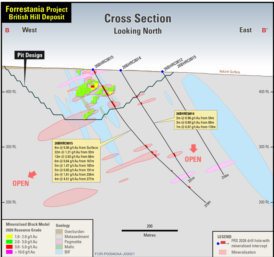
Figure 3. Cross Section B to B 1
