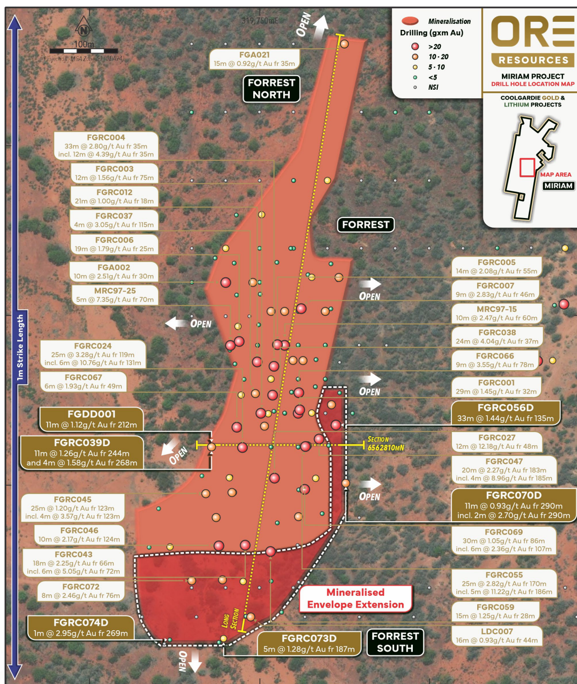
Figure 7: Forrest Plan View with significant RC and diamond drill results
