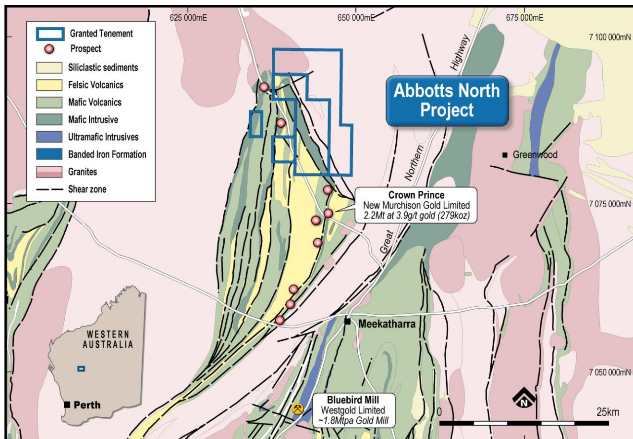
Figure 6: Abbots North project location and regional geology
