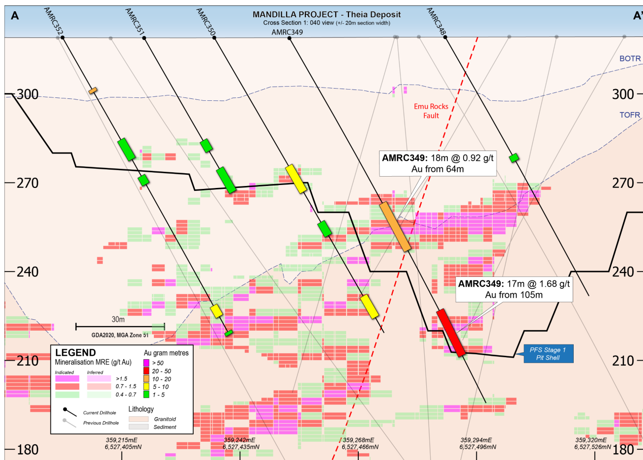
Figure 3 – Cross-section A-A' view of the Theia Deposit showing the drill trace and assay results for the current in-fill RC drilling (please note - previous drillholes are not drawn with reported assay intervals).
