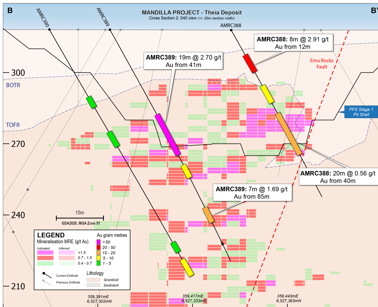
Figure 4 – Cross-section B-B' view of the Theia Deposit showing the drill trace and assay results for the current in-fill RC drilling. (please note - previous drillholes are not drawn with reported assay intervals).
