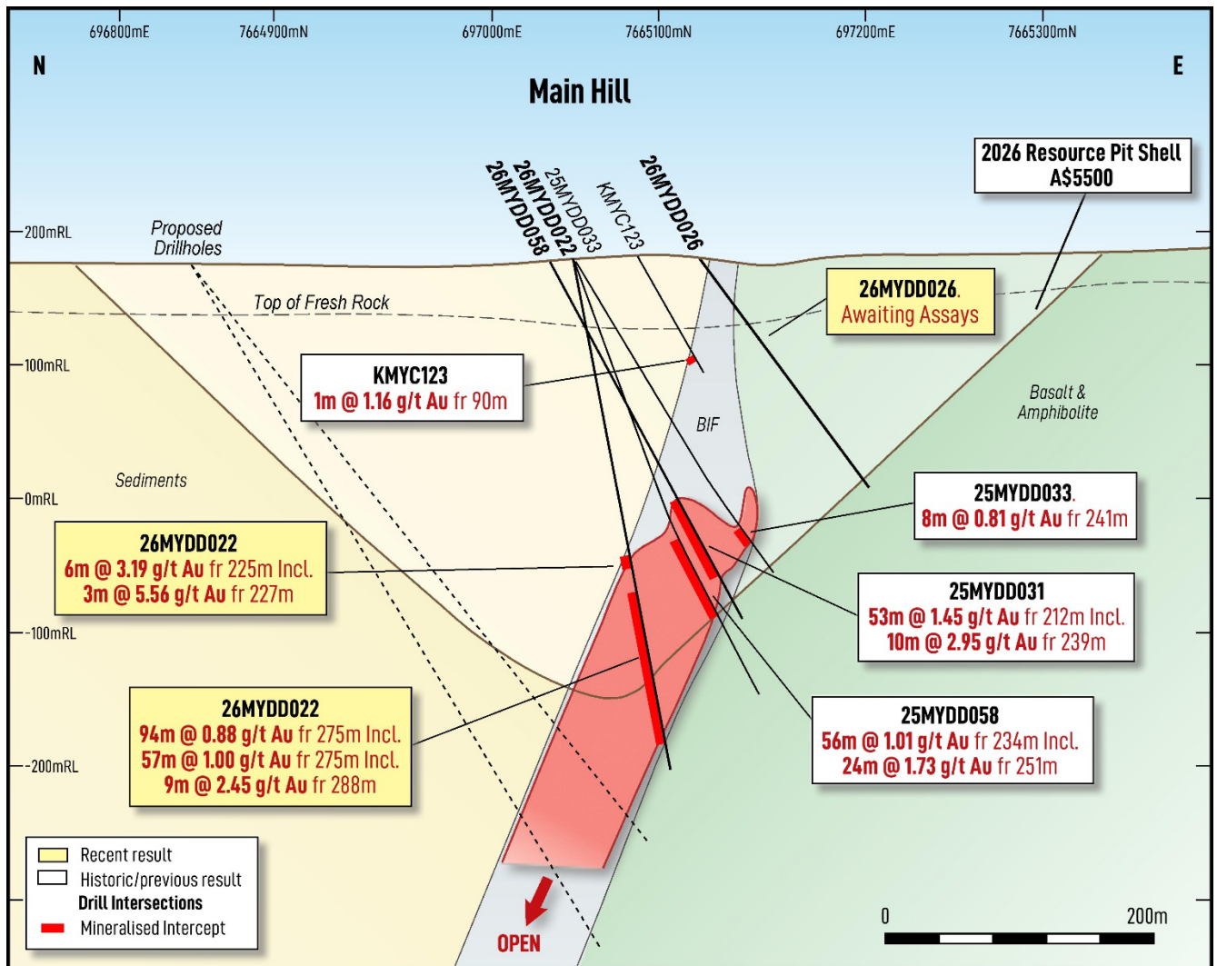
Figure 1. Cross-section through Main Hill showing the new, deeper extensional resource hole of 26MYDD022 confirming mineralisation at depth and extending mineralisation below the current resource.
