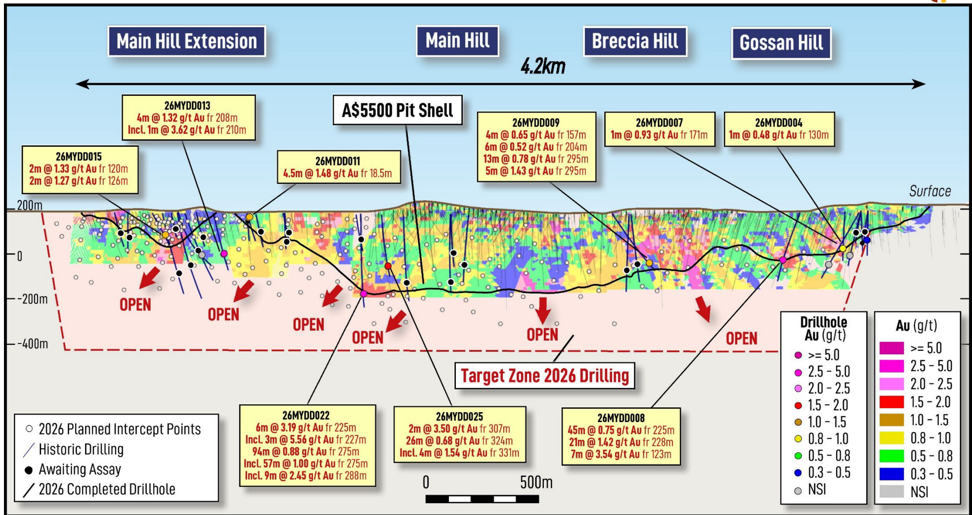
Figure 4. Long-section of the Mt York Gold Project showing all intercept points for current (yellow box) and historic drilling. Planned intercept points for 2026 drilling shown. Drilling completed (results awaited) shown as black dots with white outline.
