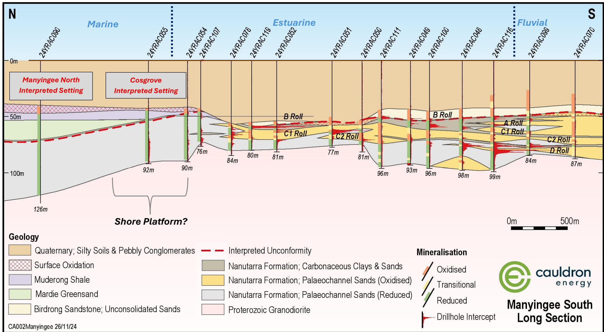
Figure 3. Manyingee South Long-Section showing the interpreted settings of mineralisation encountered at Manyingee North and Cosgrove.
