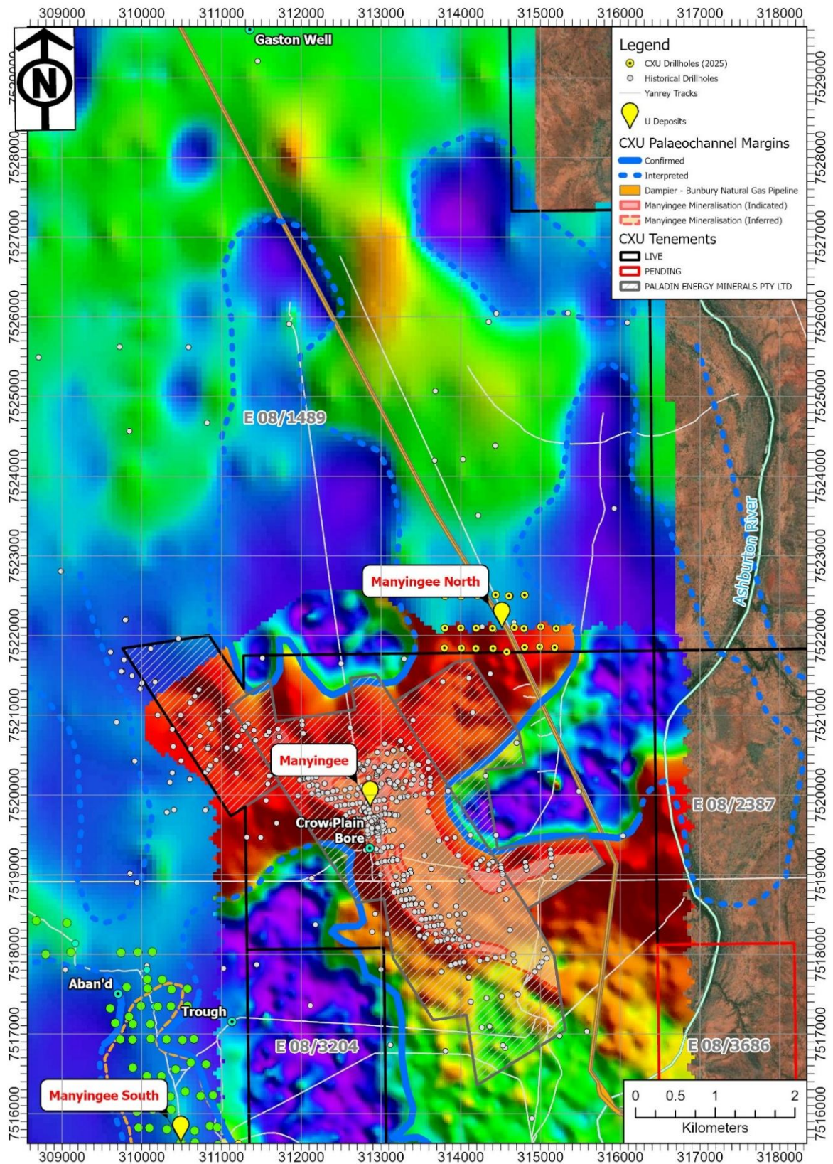
Figure 4. Combined airborne electromagnetic imagery over the Manyingee North and Manyingee palaeochannels.
