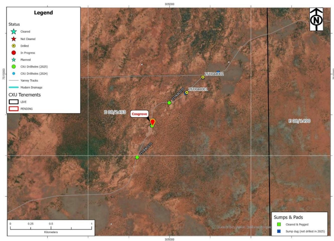
Figure 8. Exploration drillholes at the Cosgrove Prospect.
