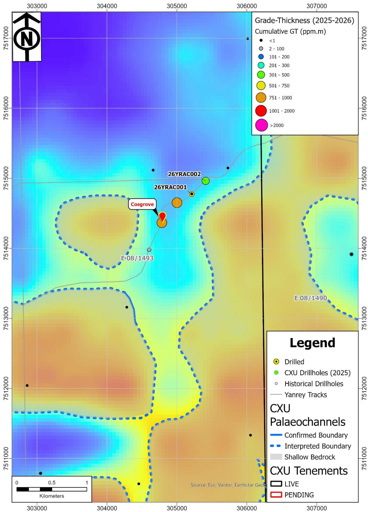
Figure 9. Cosgrove Prospect exploration drilling superimposed onto interpreted depth to bedrock surface derived from 2026 passive seismic data.
