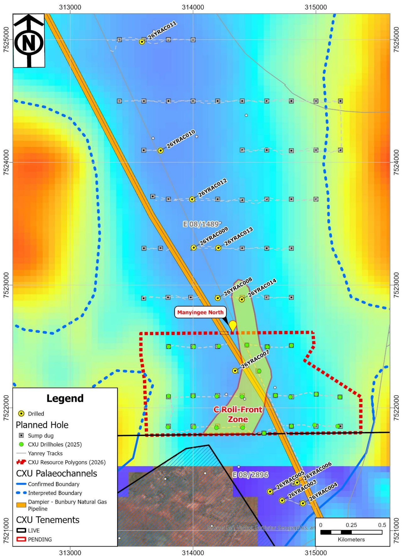
Figure 5. Manyingee North showing drillhole locations and passive seismic survey interpreted depth to bedrock surface.
