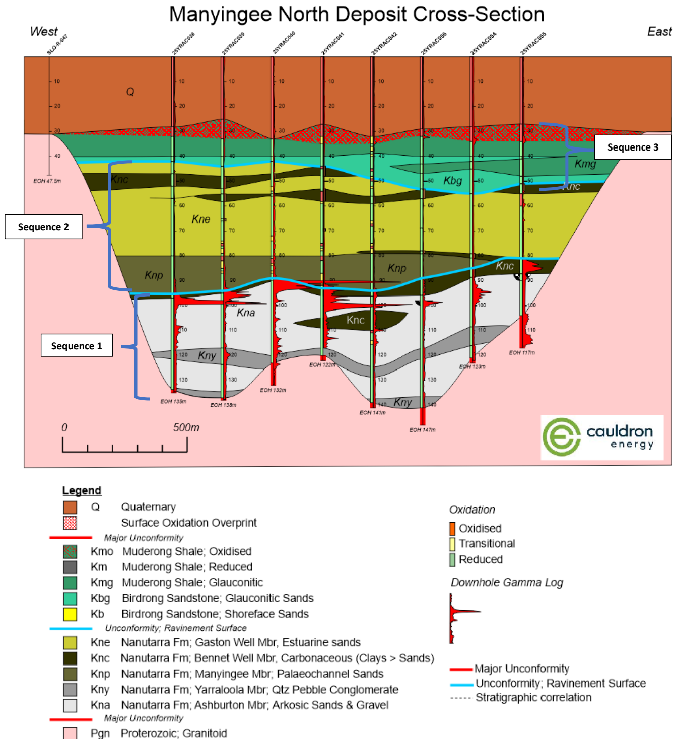
Figure 6. Manyingee North Cross-Section
