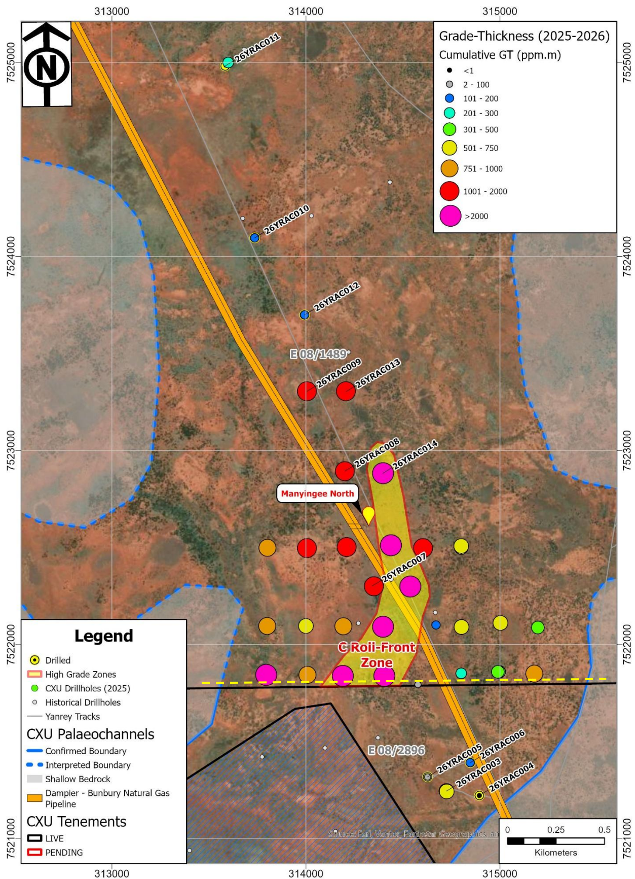
Figure 7. Manyingee North Cumulative GT (ppm*m) map. Dashed line showing location of Cross Section in Figure 6Error! Reference source not found..
