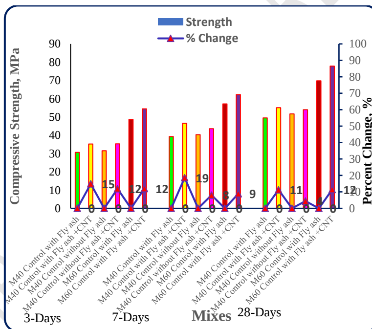
Fig. 5: Percent Increase in Compressive Strength of Concrete Mixes at different ages
