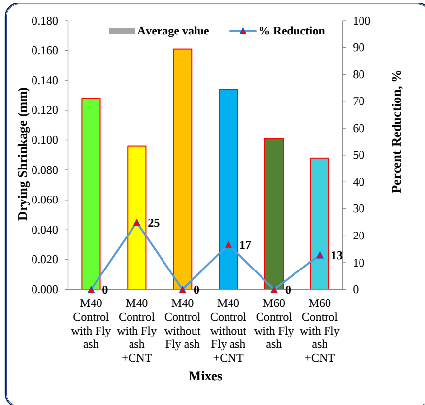
Fig. 13: Drying Shrinkage of Different Concrete Mixes
