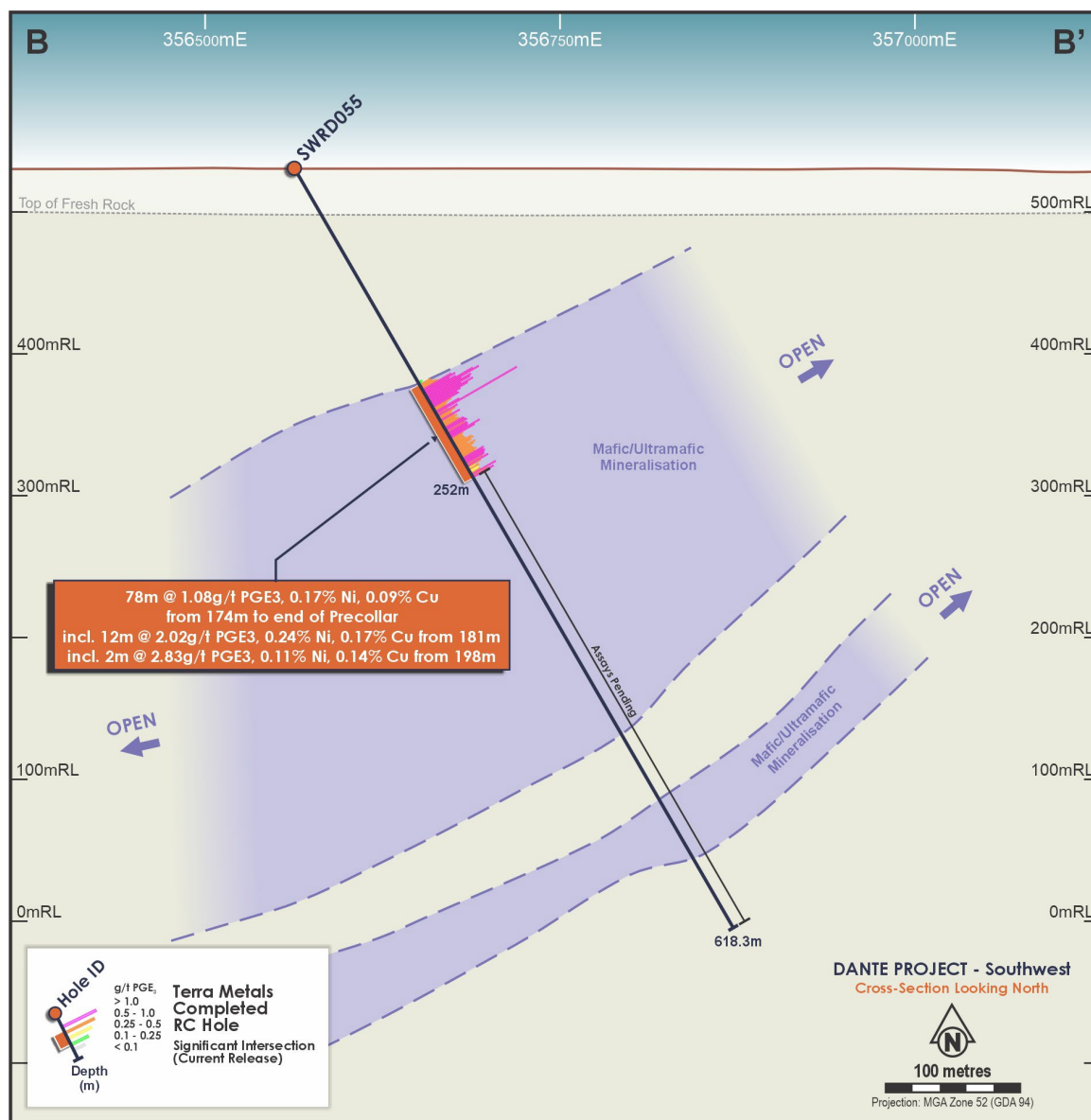
Figure 2. Cross-section B-B' through the Southwest Main Sulfide Zone showing the currently reported RC Pre-collar of SWRD055 with interpreted mineralised envelopes. The envelopes are conceptual and based on current drilling, geological logging and structural data.
