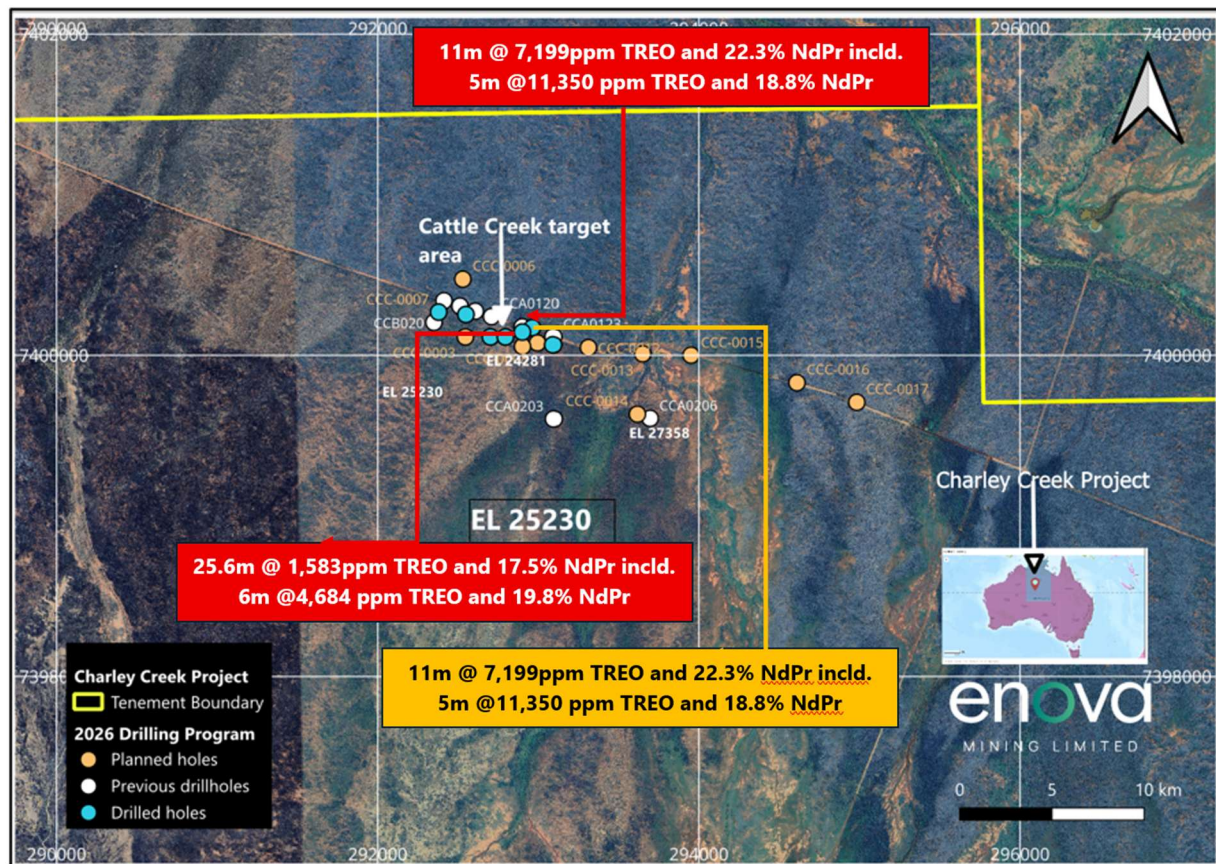
Figure 1: Air-core and diamond tail drill holes locations at the Cattle Creek Central Prospect.
