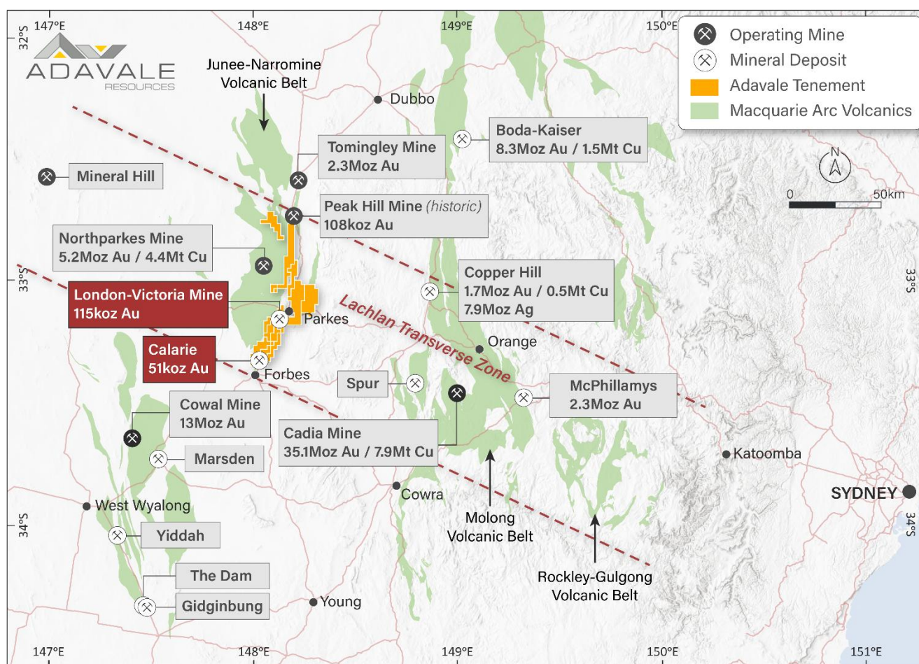
Figure 1: Map of the central New South Wales Lachlan Fold Belt
