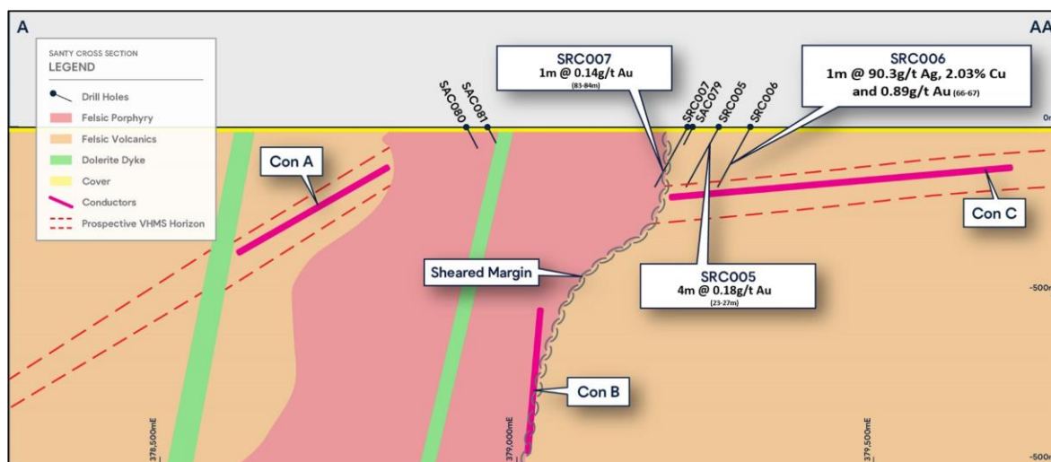
Figure 7 Cross-section of Historic MLEM Conductors and exploration results at the Santy Prospect
