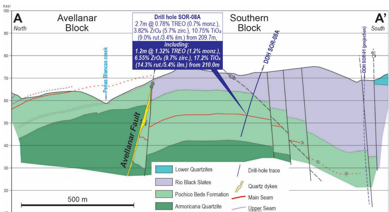
Figure 3 – SOR-08A cross-section.
