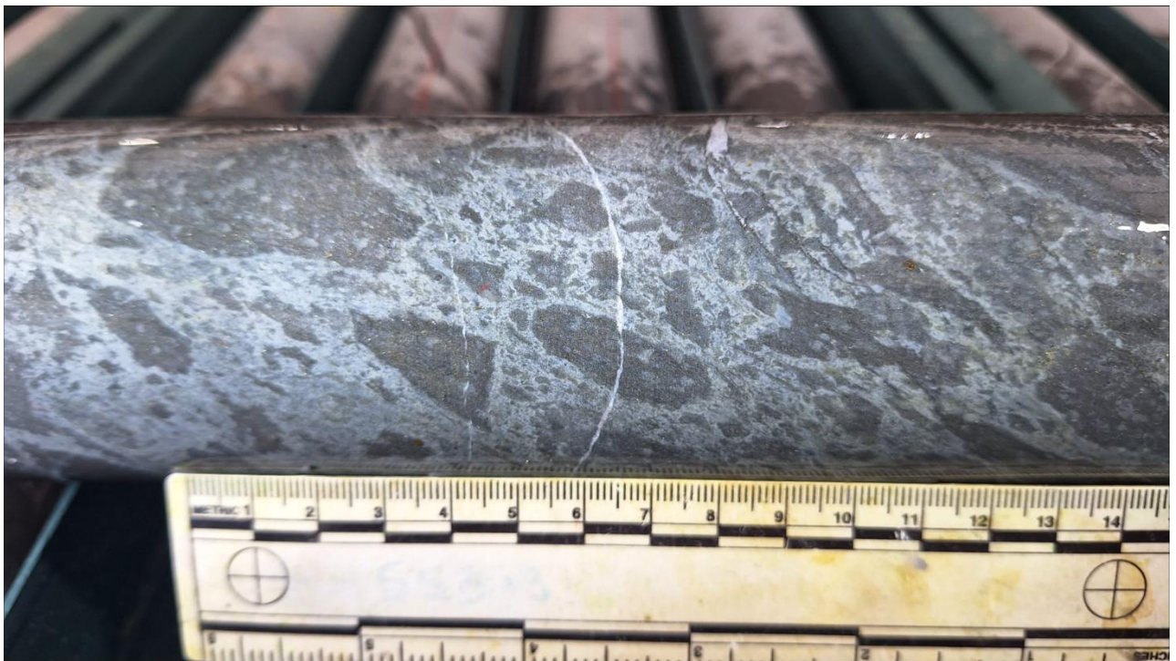
Image 3 - Pyritic rhyolite breccia 15-20% py at 1113.5m
