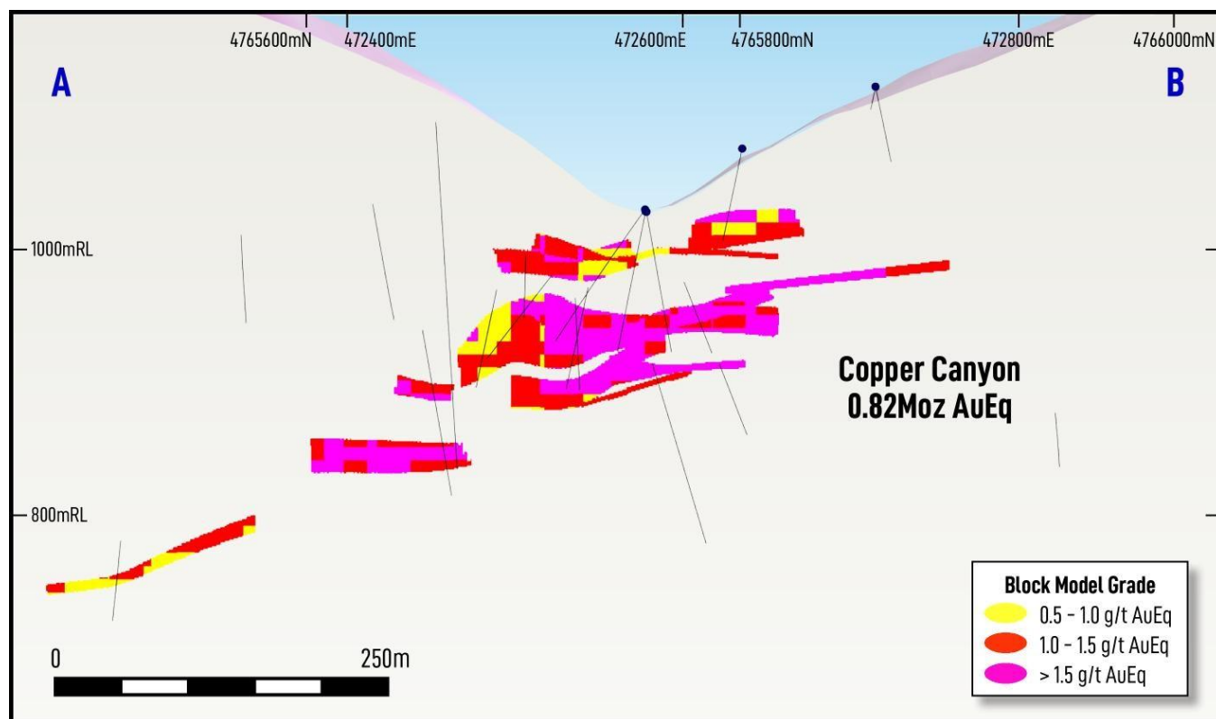
Figure 6. Copper Canyon cross-section along A – B, looking north, showing drill traces and model blocks with AuEq grades.
