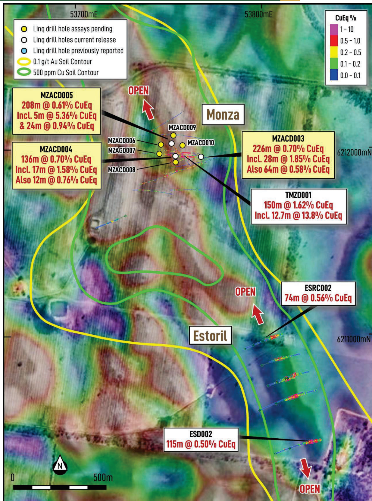
Figure 2: Monza/Estoril plan image illustrating the location of drilling results for MZACD003, 004 and 005.
