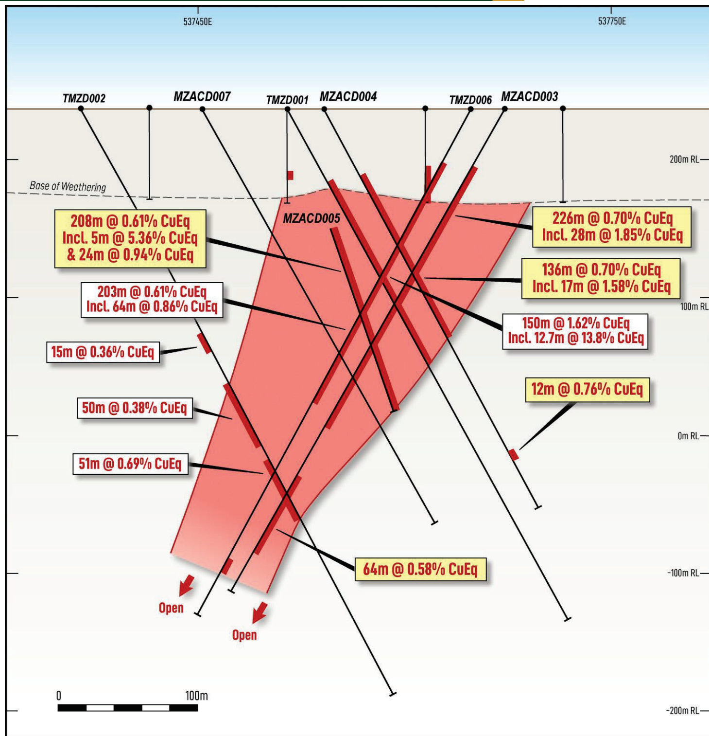
Figure 3: Monza section 6211985mN (GDA94) illustrating the location of drilling results for MZACD003, 004 & 005. MZACD007 assay results remaining pending.
