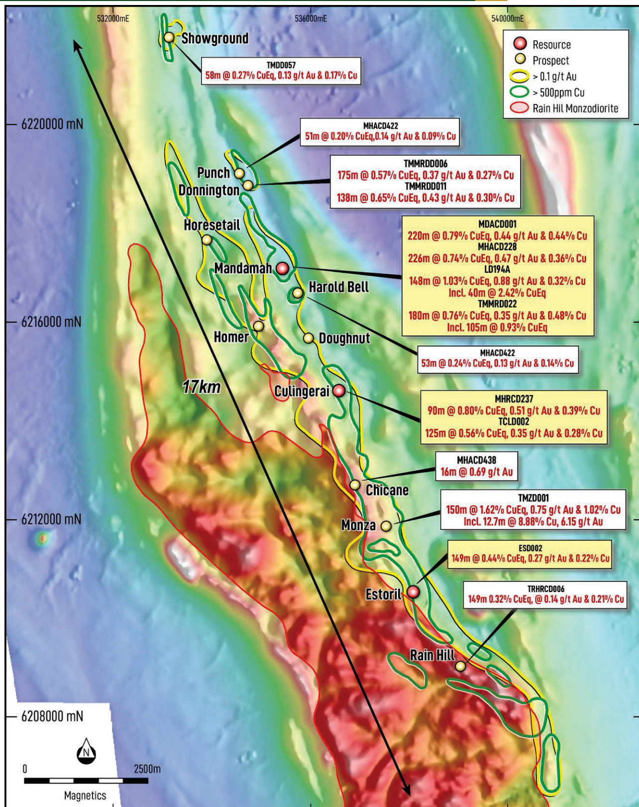
Figure 1: Central Zone resources and prospects over background reduced to pole aeromagnetic image highlighting a 17km strike.
