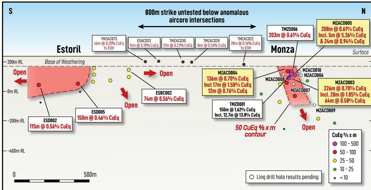
Figure 5: Estoril to Monza longsection illustrating the location of drilling results for MZACD003, 004 & 005 along with a selection of previous drill holes and also of a selection of aircore results between Estoril and Monza. MZACD006 - 010 assay results remain pending.
