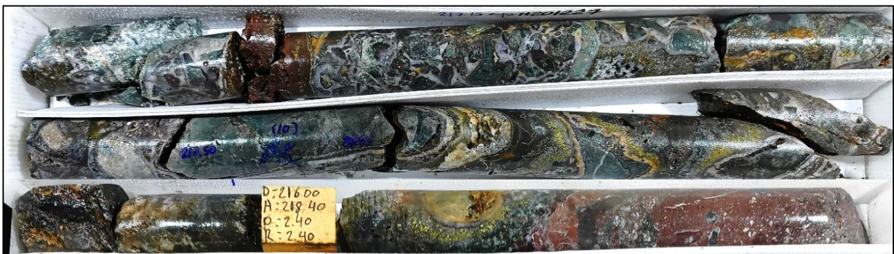
Figure 4. Complex quartz-sulphide breccia zone from ~217 metres downhole in GV-26-003 showing strong chalcopyrite veining (yellow) developed in multiple areas. This interval includes a high grade zone of 1.9 metres at 3.0% Cu, 155g/t Ag & 1.9g/t Au from 217.2m.
