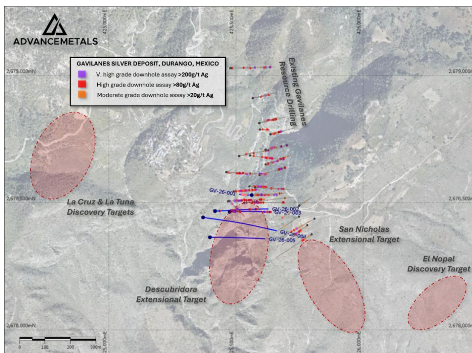
Figure 1. Plan view of the Gavilanes Project showing previous drill holes with downhole silver grades 5 along with Advance's key drilling targets. The location of recent AVM drill holes GV-26-001 to GV-26-005 are also shown on the plan.
