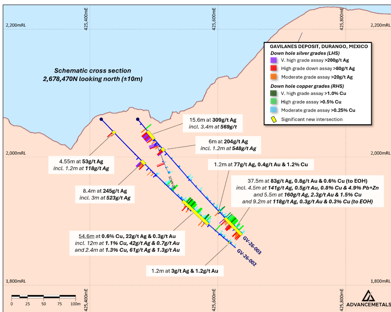
Figure 3. Schematic cross section at 2,678,470N showing downhole silver and copper grades and significant intersections returned from Advance Metals' holes GV-26-002 3 and GV-26-003 at the Gavilanes Project, in reference to previous drilling 5 .
