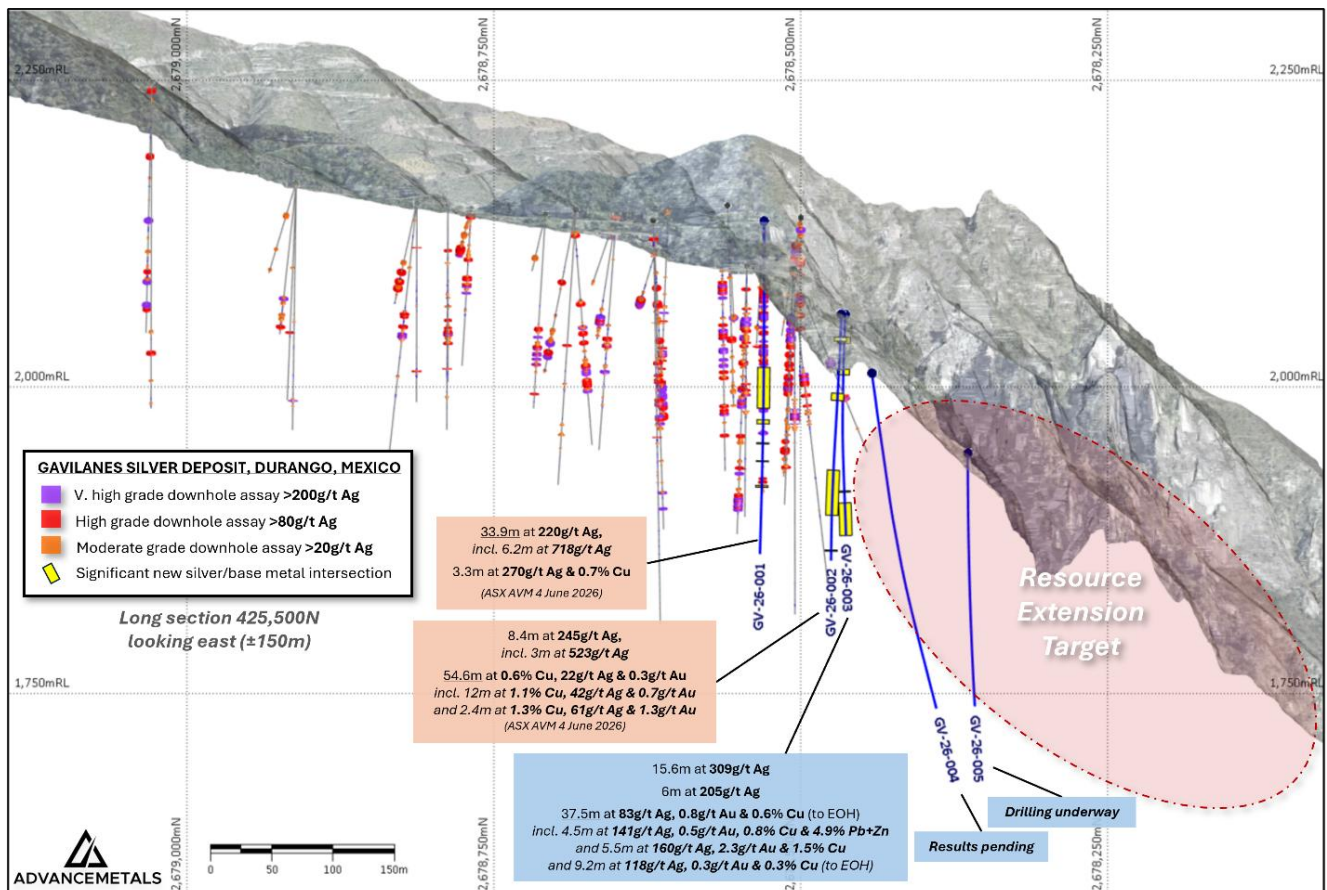
Figure 4. Long section showing previous drilling with downhole silver grades 5 at Gavilanes along with Advance's recent drill holes (blue) and results at the southern end of the high grade system.
