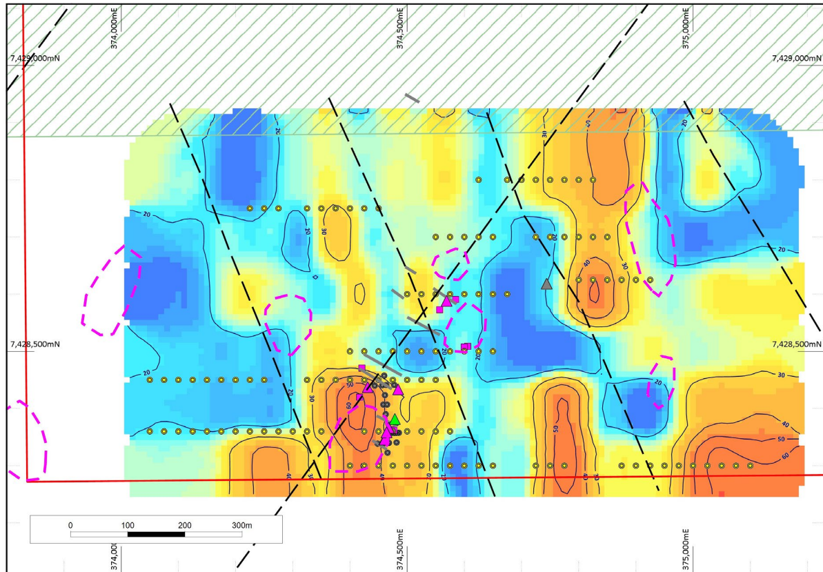
Figure 5. Copper in soils (contour interval 10ppm) and residual gravity anomalies (pink dashed outlines).
