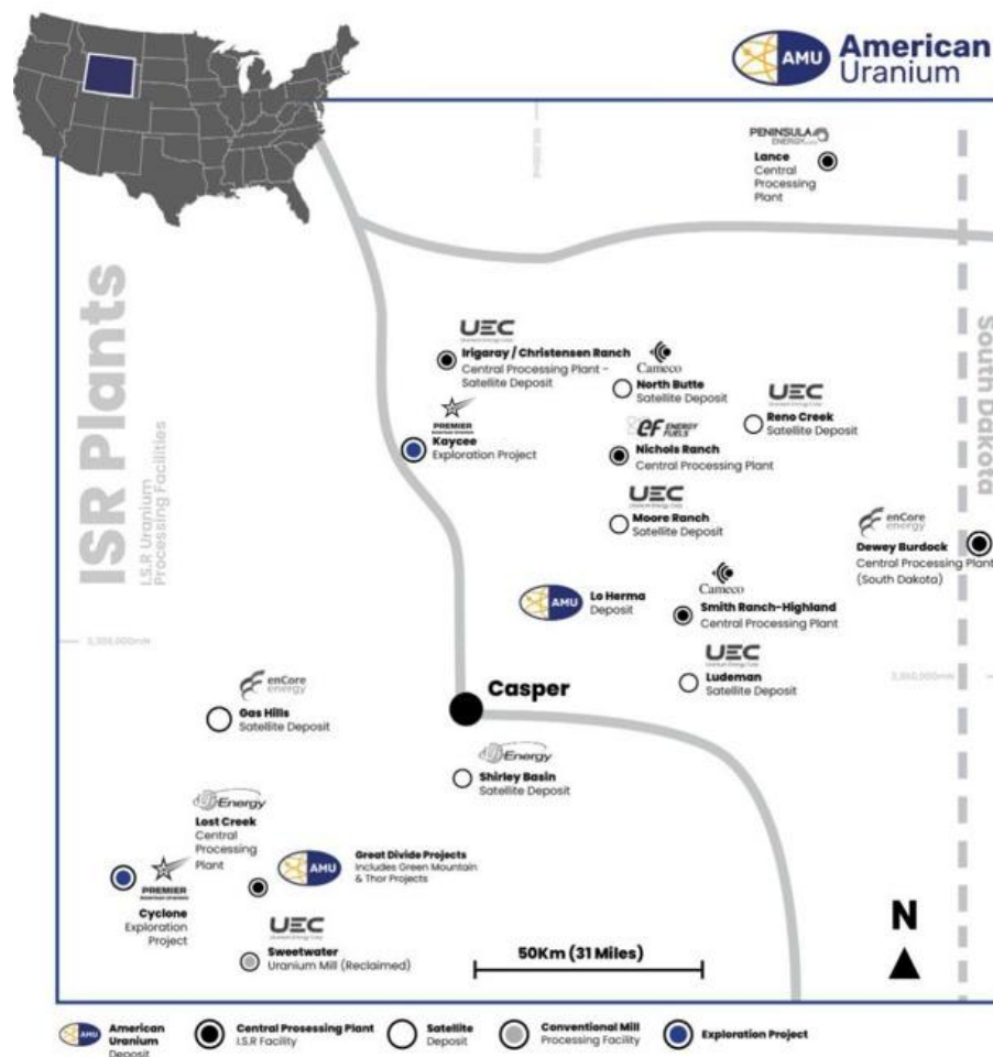
FIGURE 5. WYOMING ISR URANIUM ASSETS & AMU PROJECT LOCATIONS
